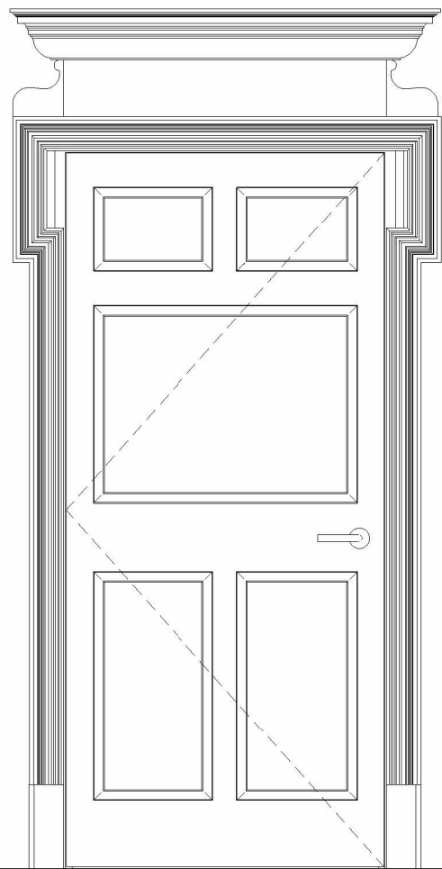
Door Type A1 5 panelled door leaf only L20 / 409
