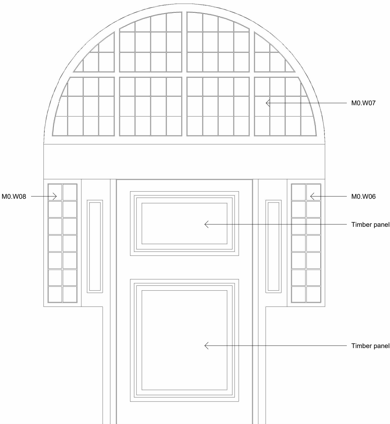
Door M0.D01 Illustrative elevation as viewed internally Existing door retained
