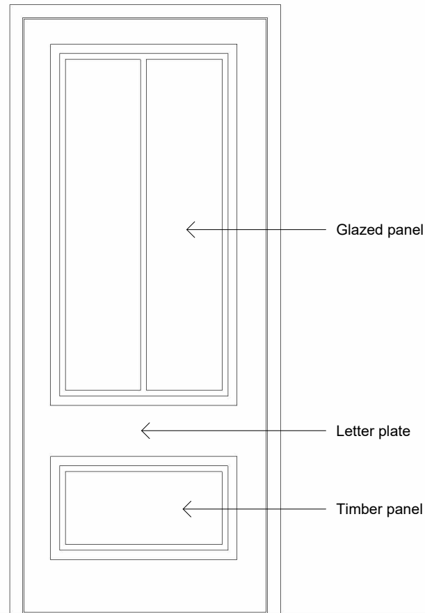
Door L0.ND10 L20 / 412A Illustrative elevation as viewed externally
