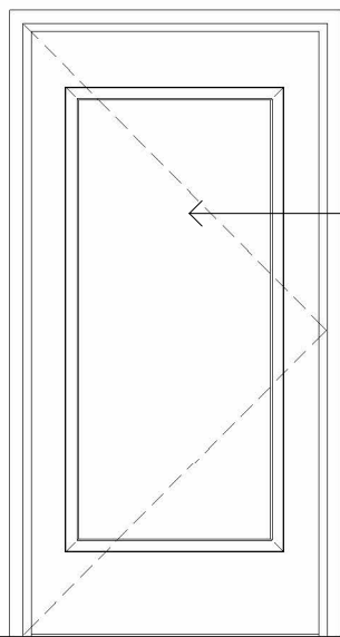
Door Type E Single panelled door leaf only L20 / 409
