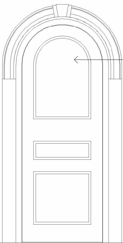
Door Type C1 3 panelled door leaf only arched head L20 / 409 Architrave shown as door M1.D01
