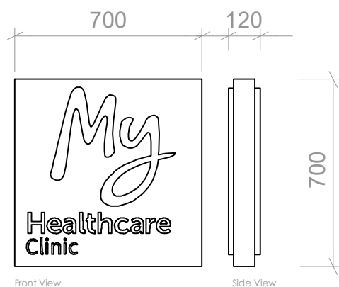
Proposed Projecting Signage 1:20
