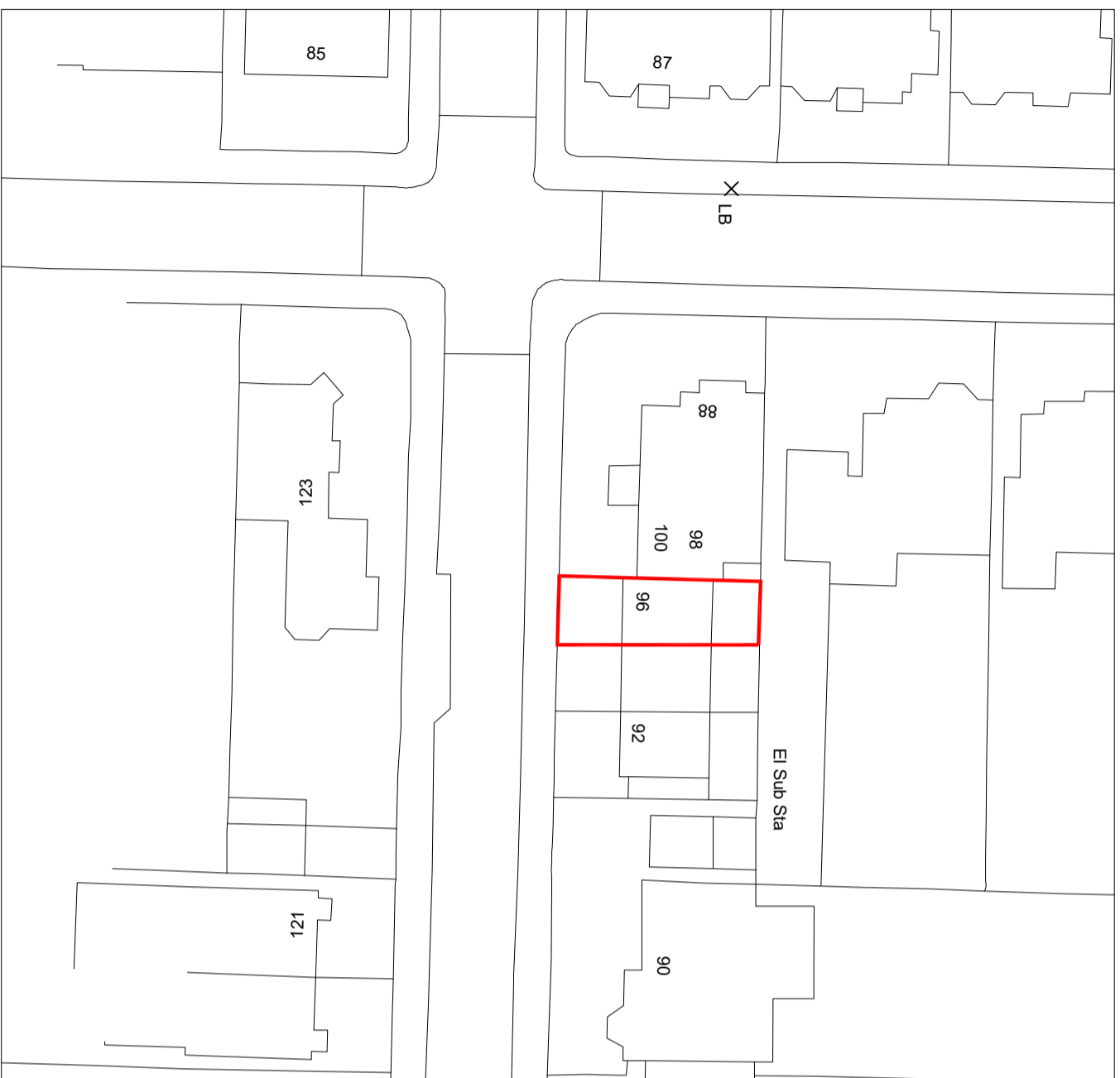
BLOCK PLAN 1:500
