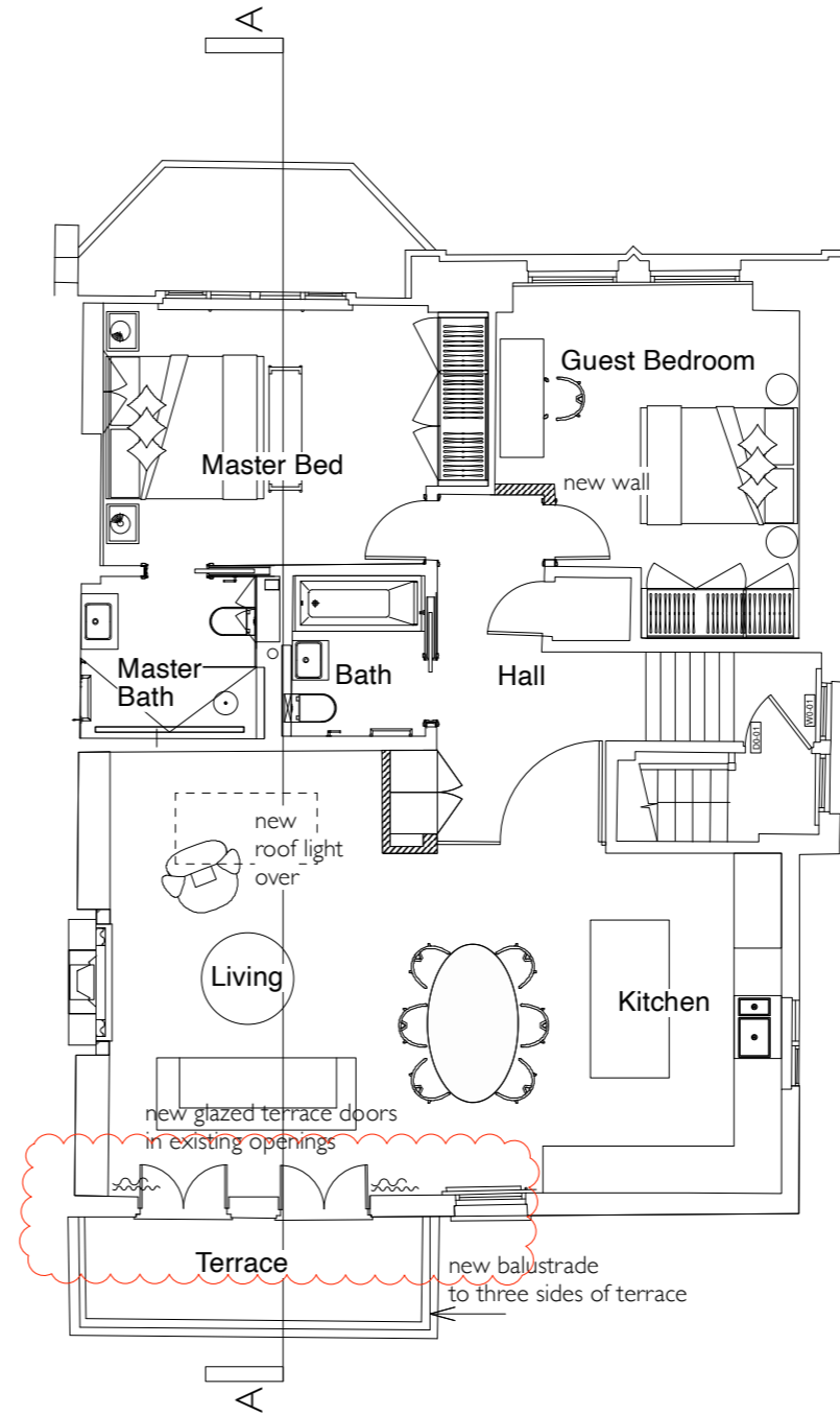
2 Proposed Plan 1:100
