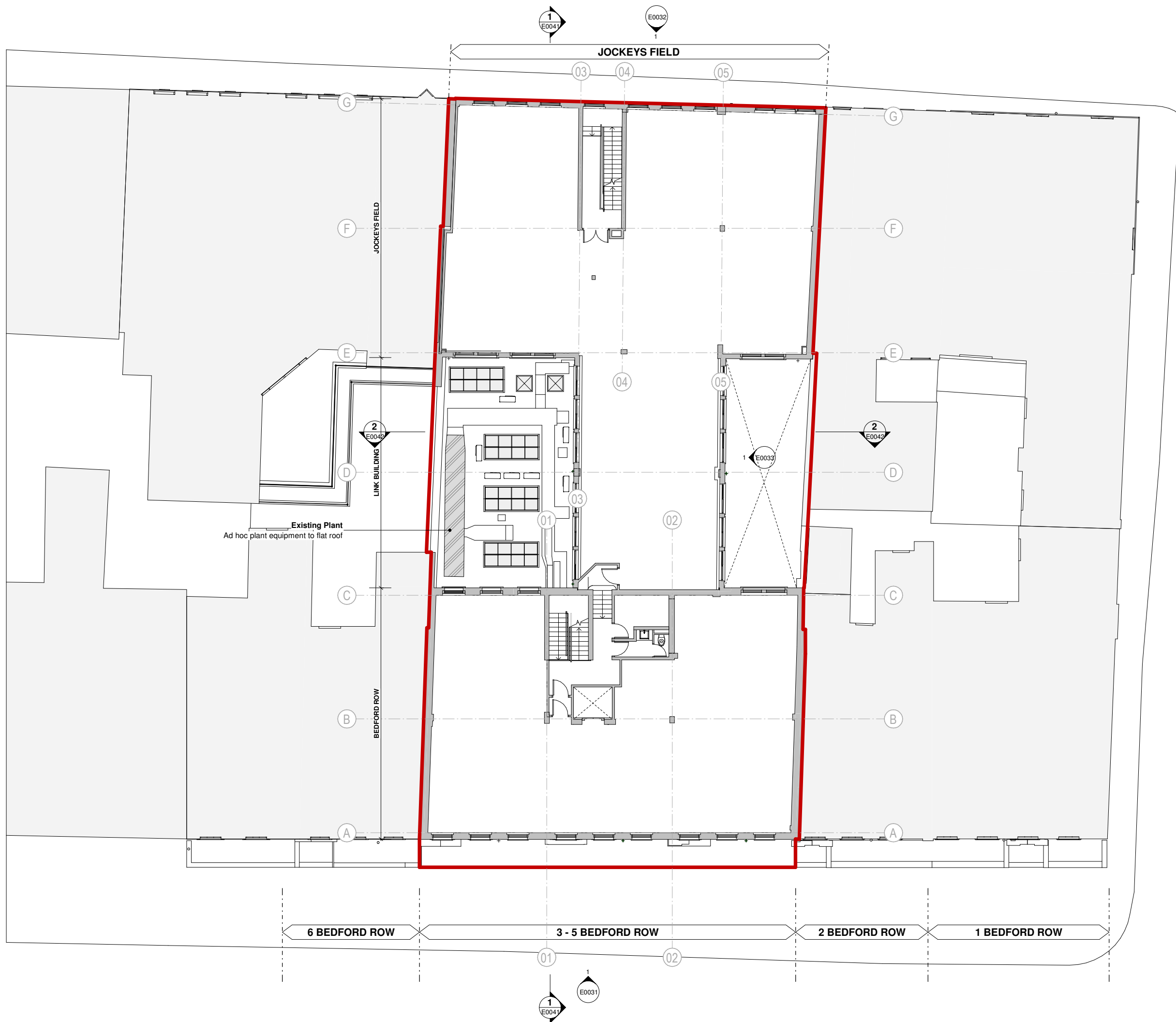
E0011 - B - Existing First Floor
