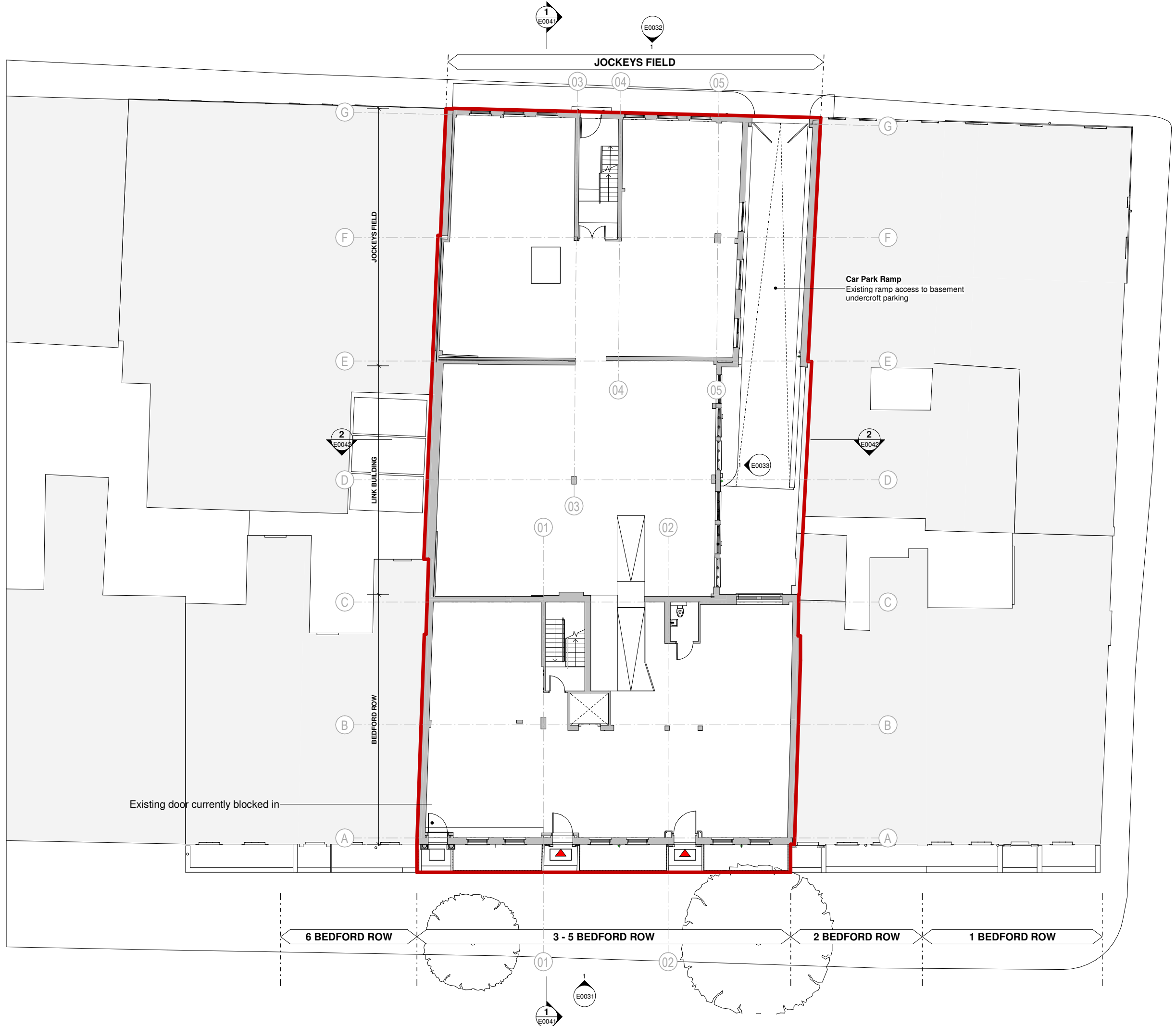
E0010 - B - Existing Ground
