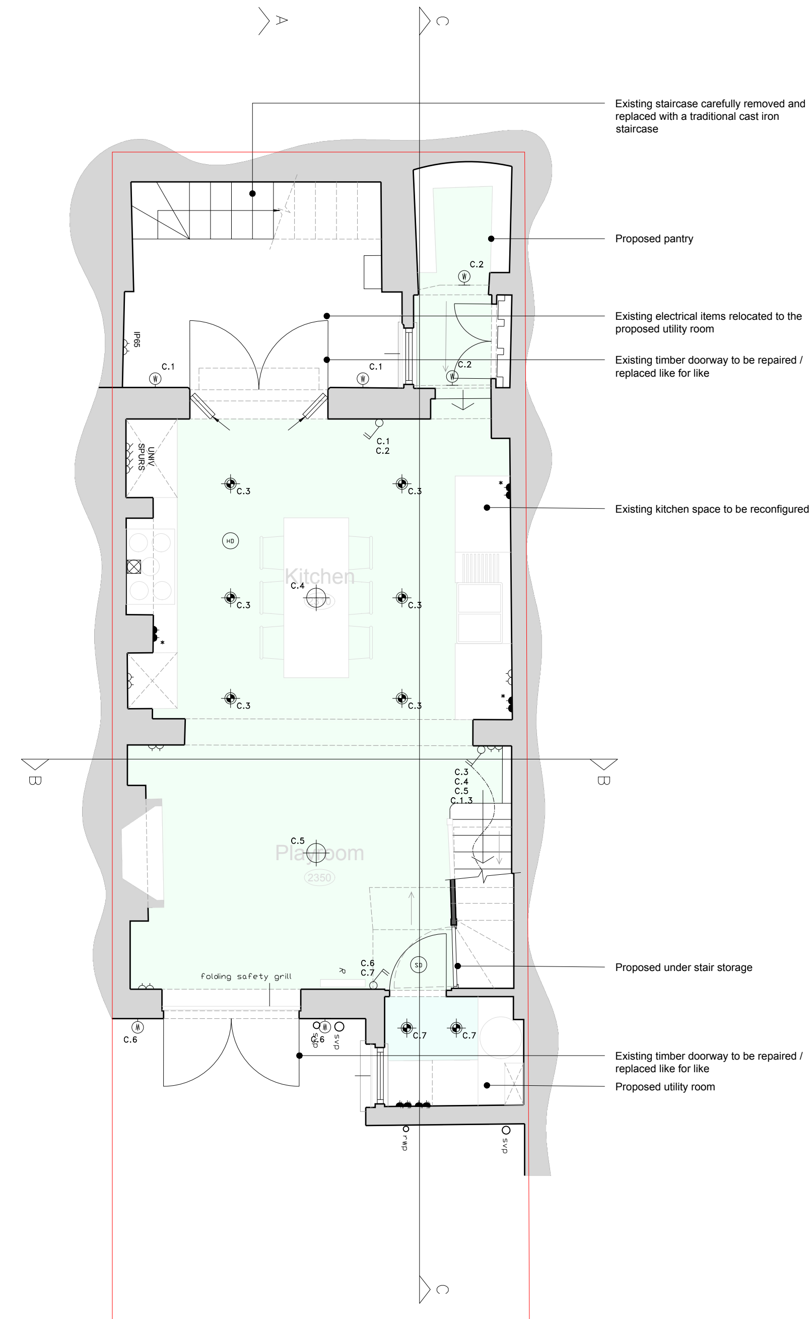
PROPOSED LOWER GROUND FLOOR PLAN
