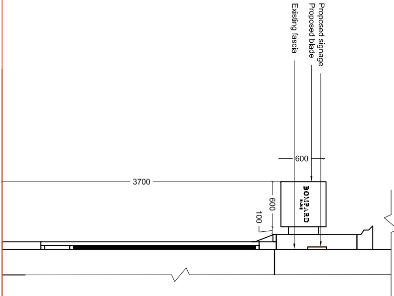
Section A-A As Existing - Scale 1:50
