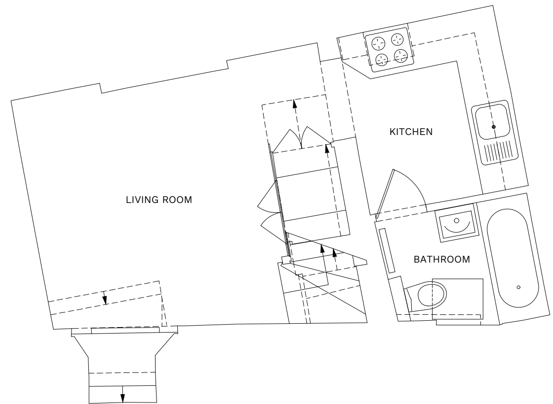
3 EXISTING LOWER PLAN 1:50 / A3
