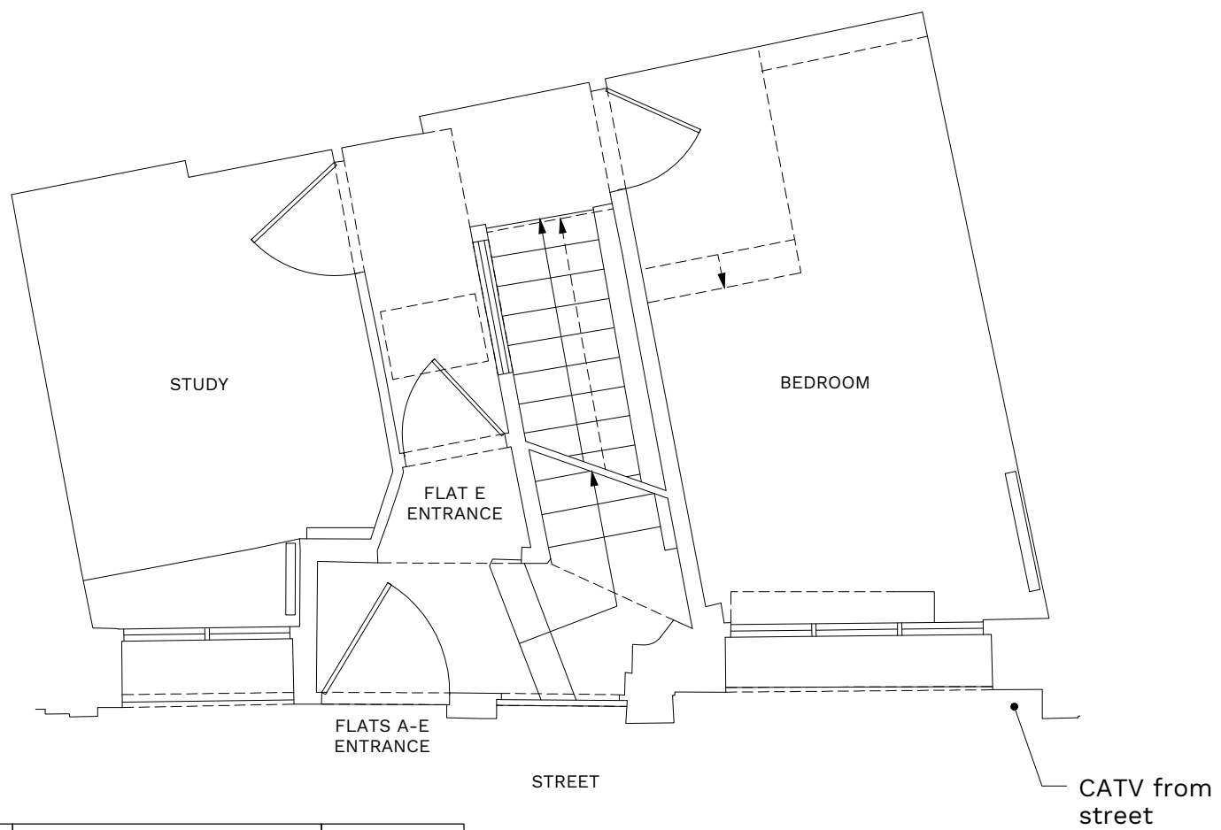
2 EXISTING GROUND PLAN 1:50 / A2
