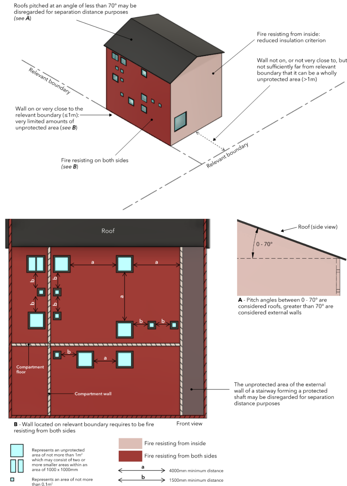
Figure 13 - Exclusion from unprotected area calculations
