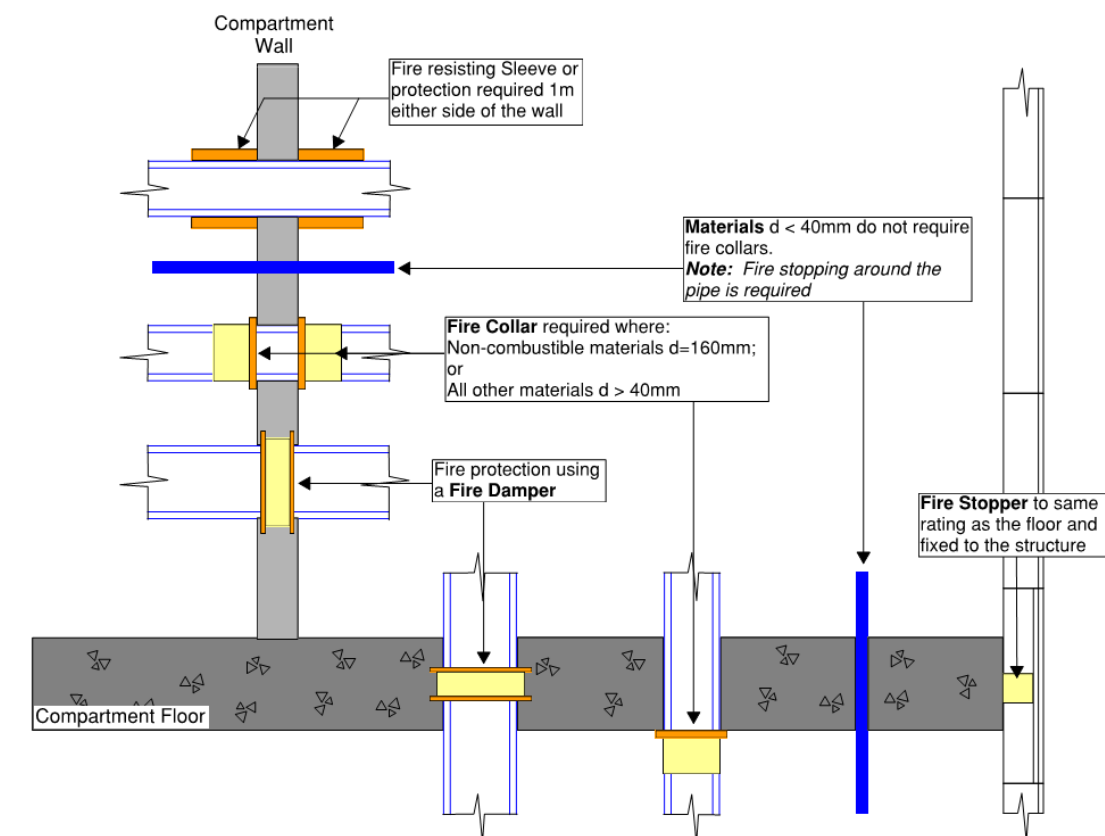
Figure 11 – Fire-stopping expectations
