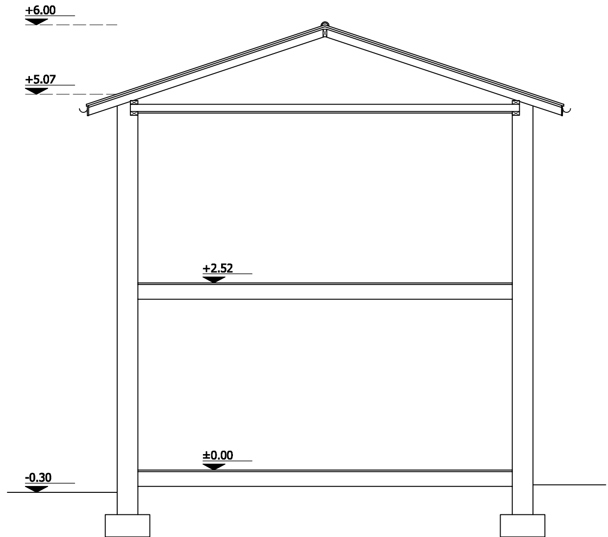
EXISTING SECTION scale 1:50
