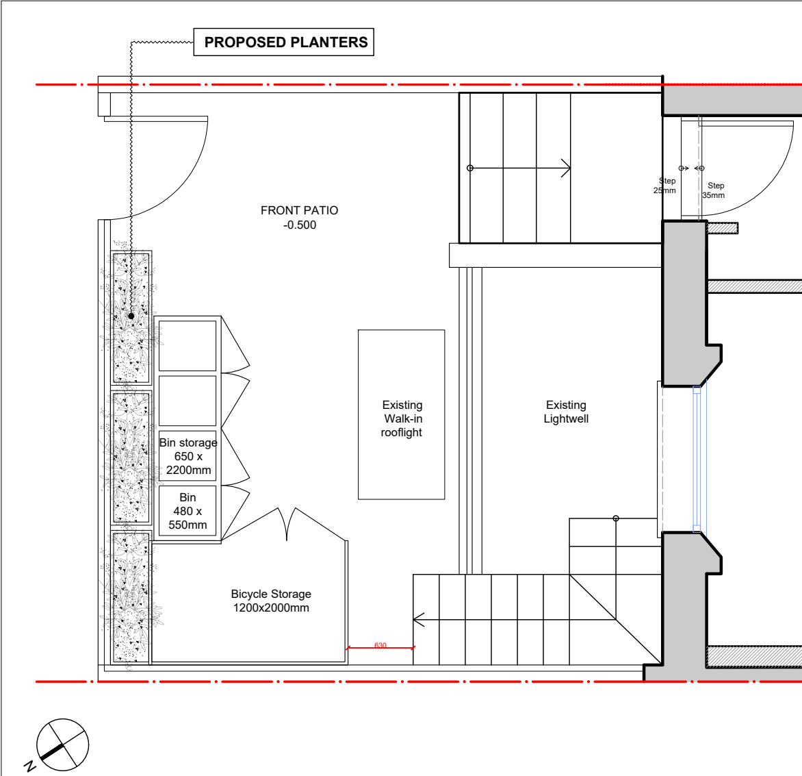
2 Scale: 1:50 @ A1 PROPOSED FRONT GARDEN PLAN
