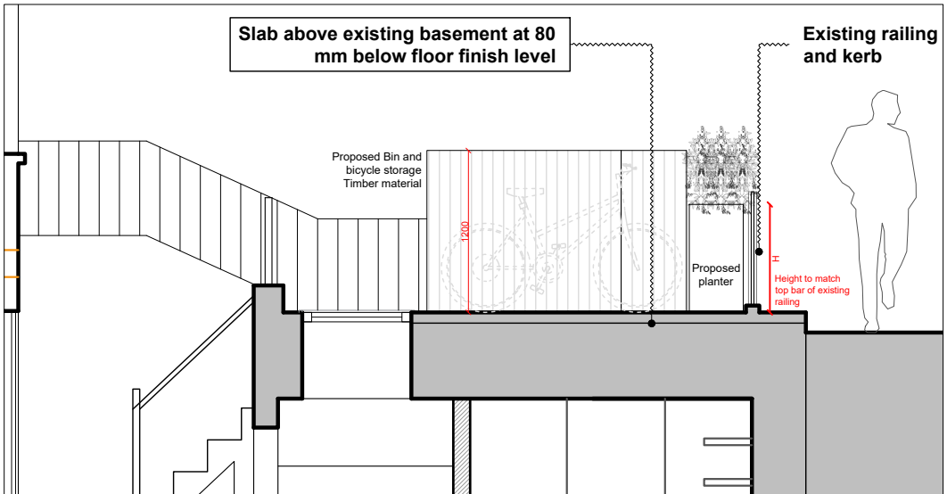
5 Scale: 1:50 @ A1 PROPOSED SIDE VIEW
