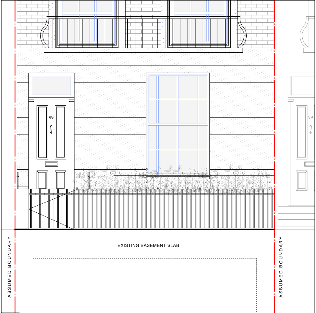
4 Scale: 1:50 @ A1 PROPOSED FRONT ELEVATION
