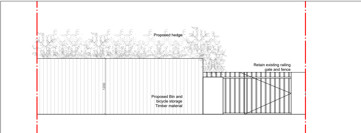
3 Scale: 1:50 @ A1 PROPOSED ELEVATION - INTERNAL VIEW
