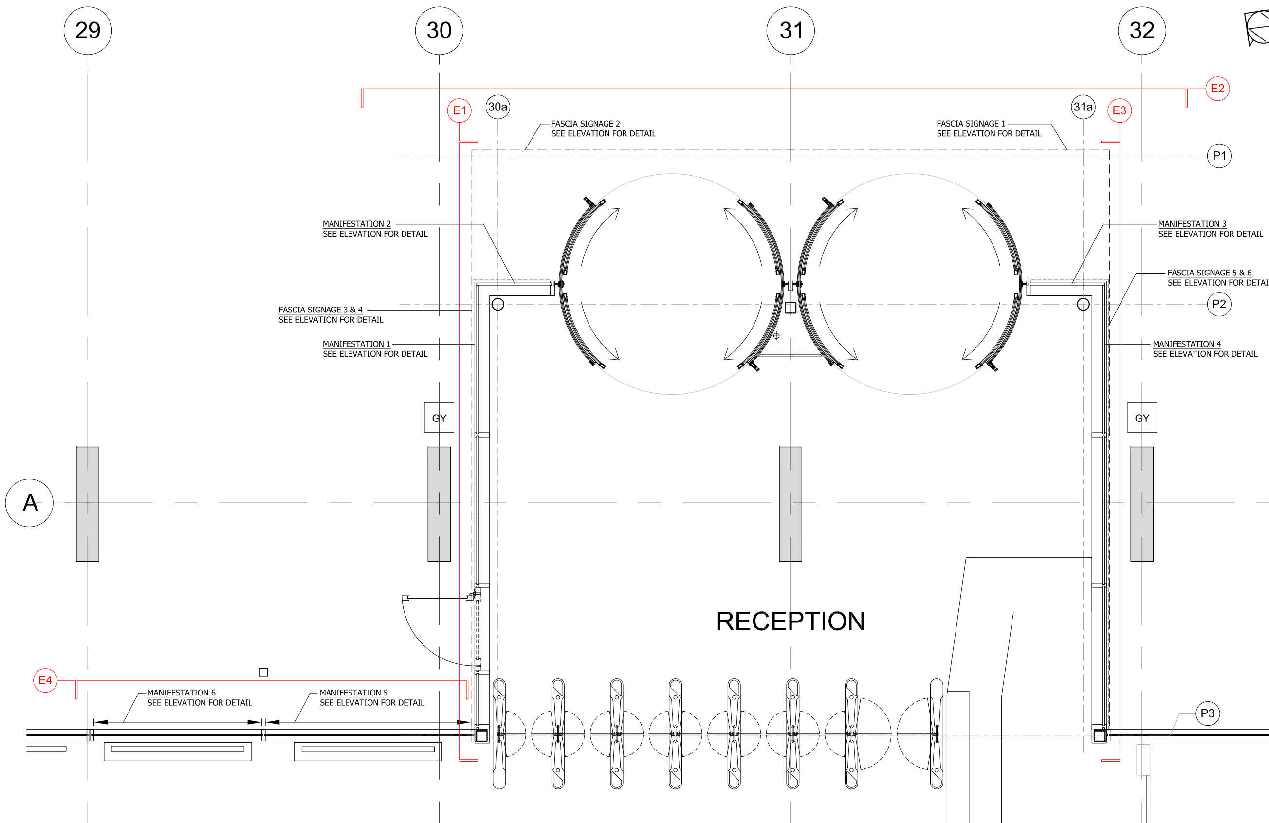
1 L3 Pavilion - As Built Proposed Signage Locations 1:50 @ A3
