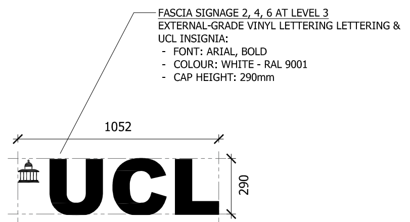
5 Fascia Signage 2, 4 & 6 Proposed Signage 1:20 @ A3
