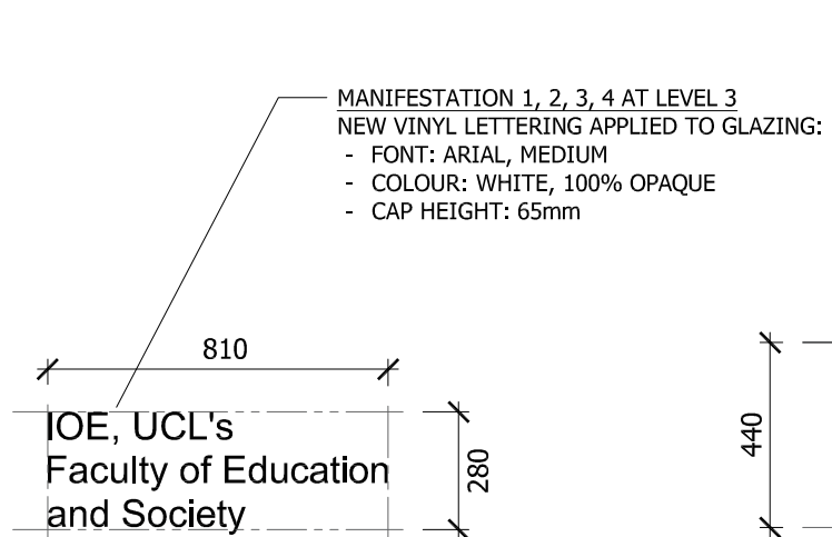
1 Manifestation 1,2,3,4 Proposed Signage 1:20 @ A3
