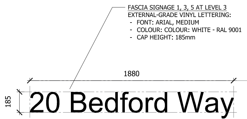
4 Fascia Signage 1, 3 & 5 Proposed Signage 1:20 @ A3
