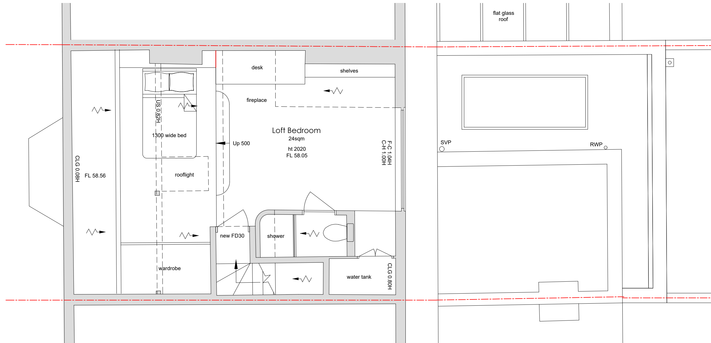
1 PROPOSED SECOND FLOOR PLAN SCALE 1:50
