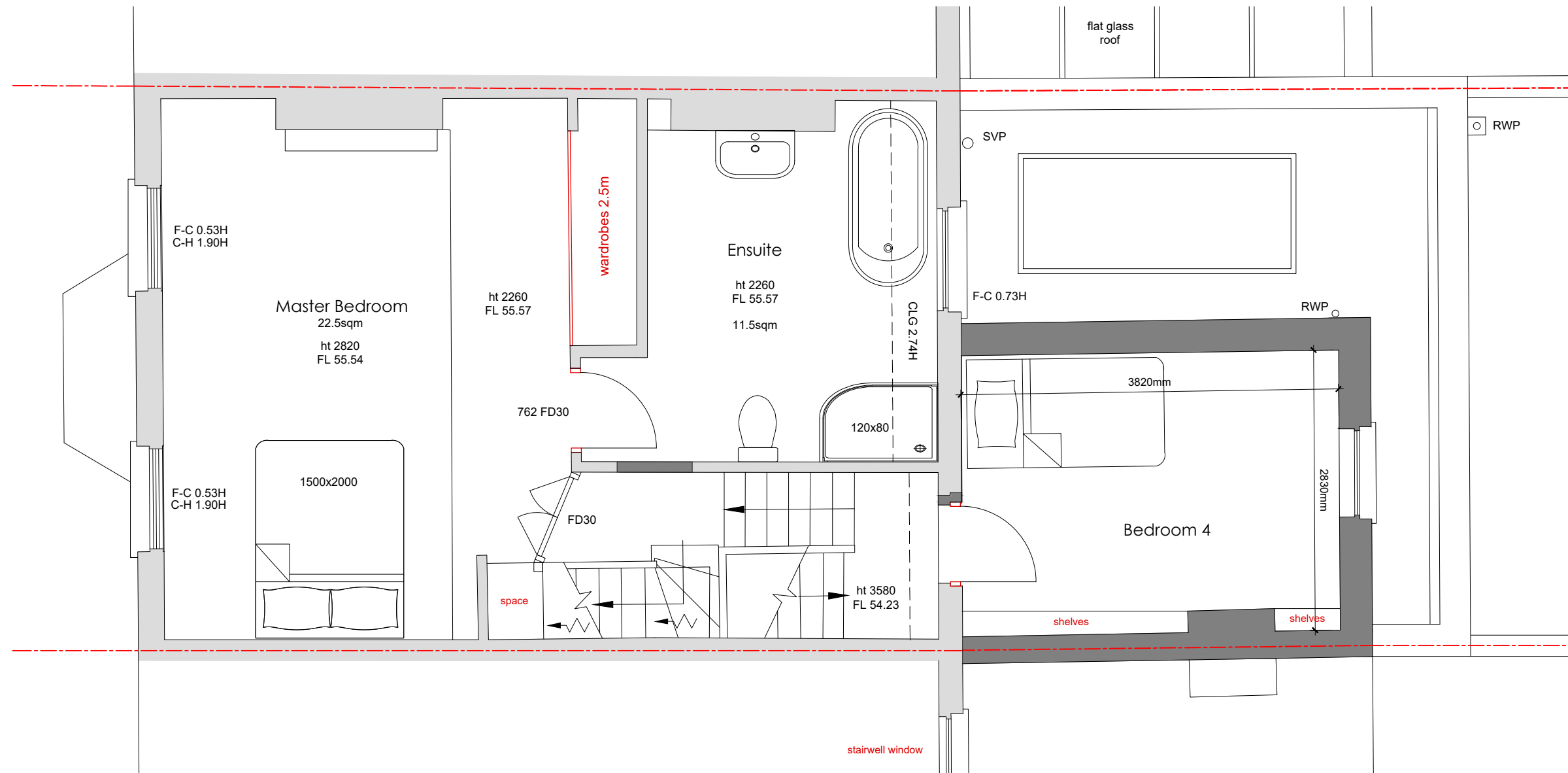
1 PROPOSED FIRST FLOOR PLAN SCALE 1:50
