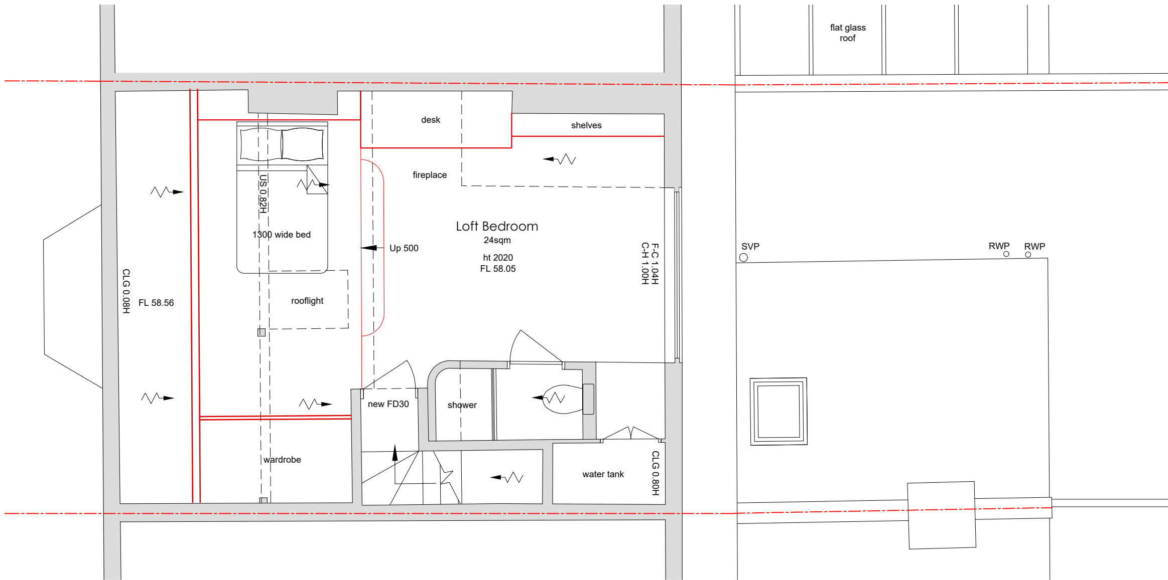
1 EXISTING SECOND FLOOR PLAN SCALE 1:50
