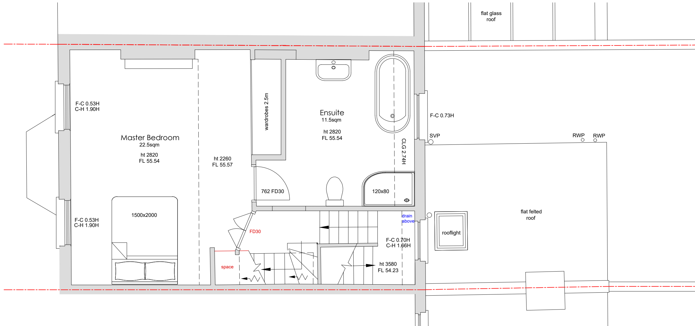
1 EXISTING FIRST FLOOR PLAN SCALE 1:50
