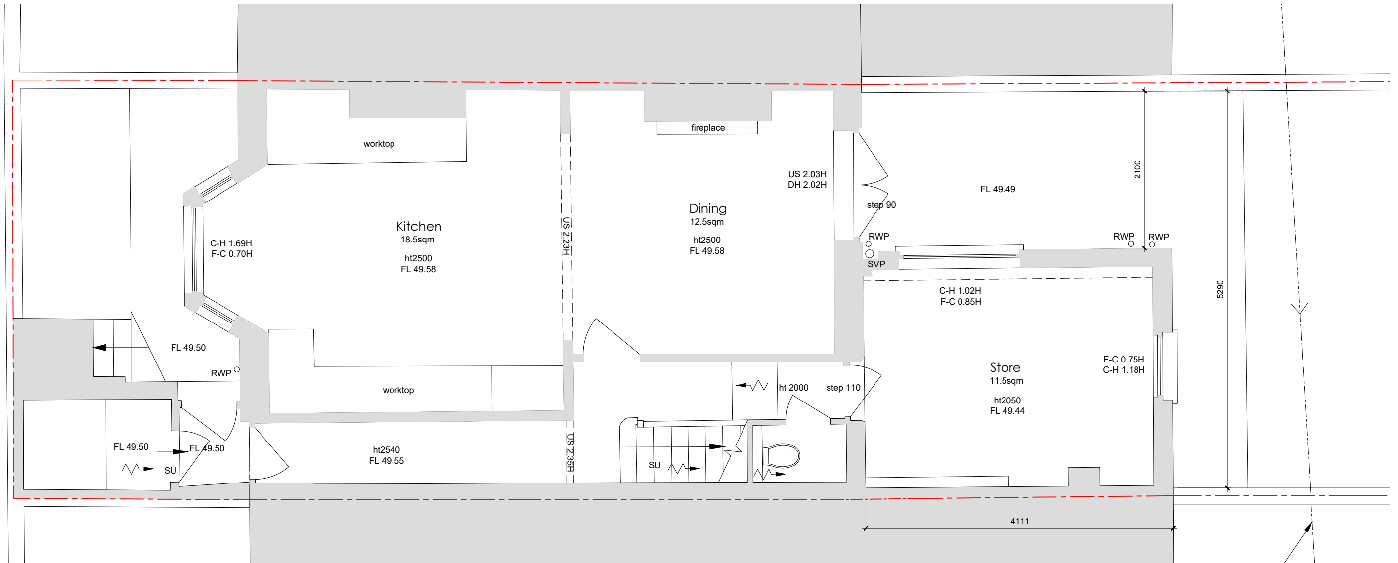
1 EXISTING LOWER GROUND FLOOR PLAN SCALE 1:50
