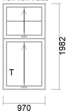
11) Sliding Sash window 145mm 1505 x 1982 View from inside
