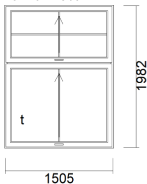
12) Sliding Sash window 145mm 970 x 1982 View from inside
