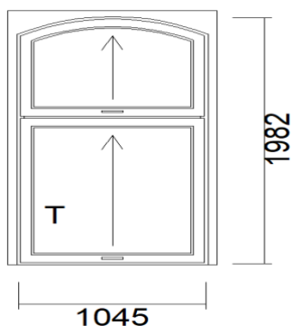
9) Sliding Sash window 145mm 970 x 1982 View from inside
