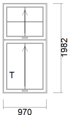
13) Sliding Sash window 145mm 920 x 1982 View from inside
