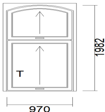
10) Sliding Sash window 145mm 970 x 1982 View from inside
