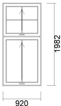
15) Sliding Sash window 145mm 986 x 1852 View from inside
