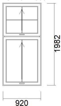
14) Sliding Sash window 145mm 920 x 1982 View from inside
