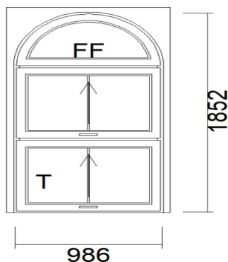
16) Sliding Sash window 145mm 976 x 1852 View from inside
