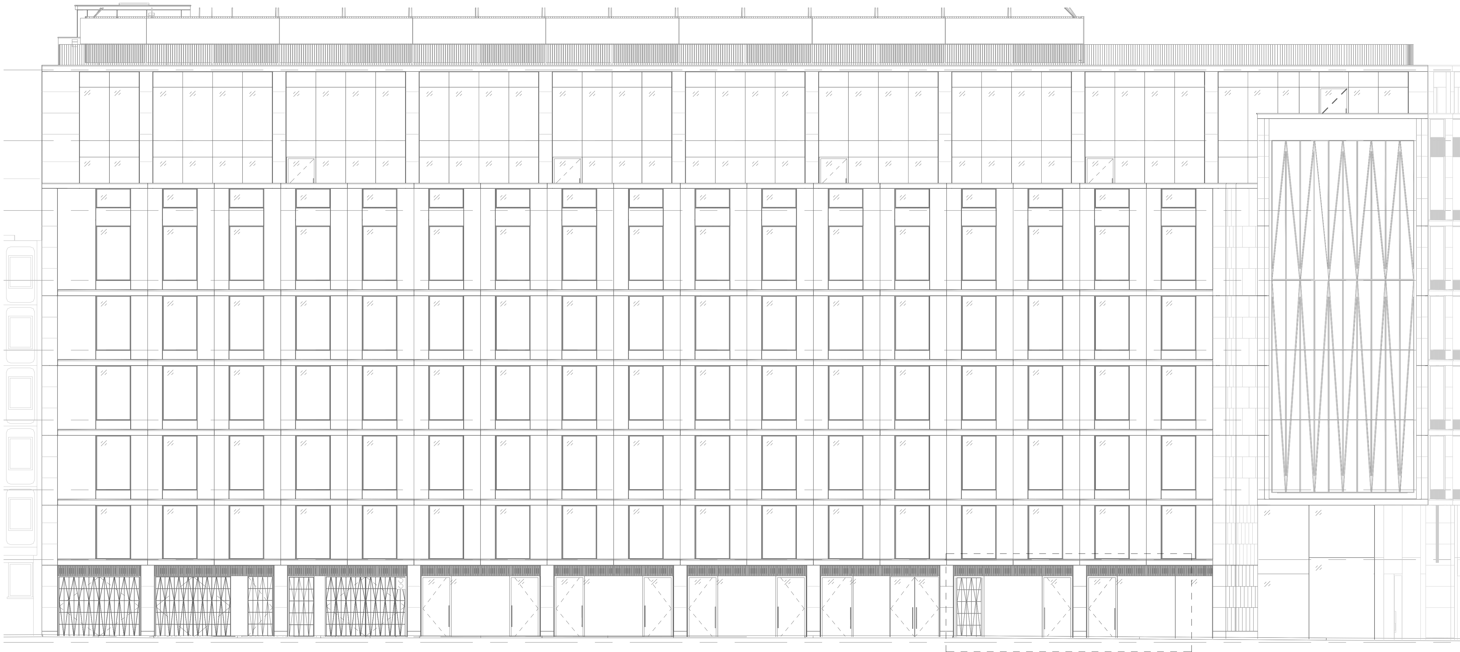
2 Proposed Drummond Street Facade Elevation
