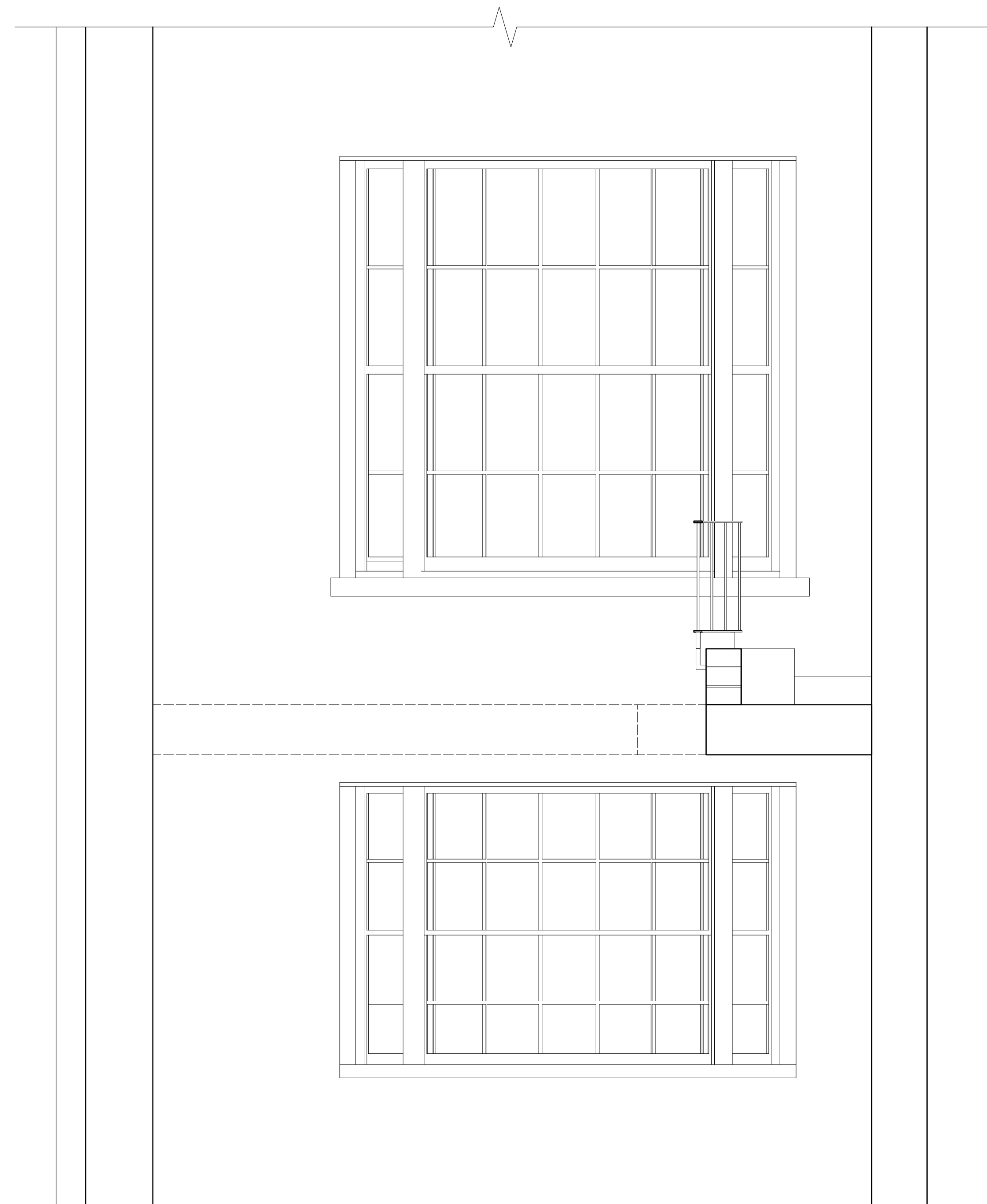
EXTERNAL ELEVATION PRIOR TO BOW WINDOW FAILURE 9 MONTAGUE ST BOW WINDOW
