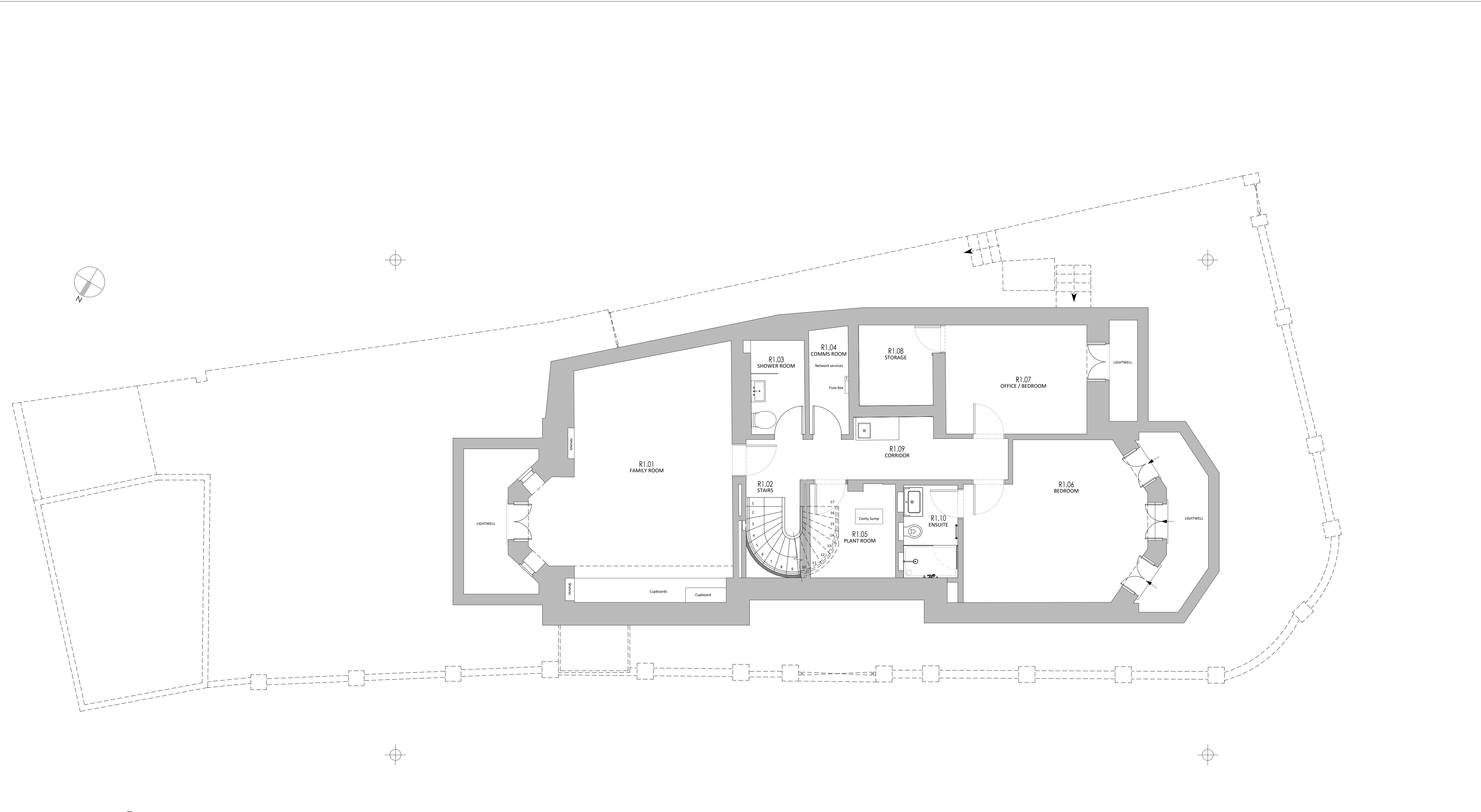
01 Existing Lower Ground Floor Plan A2.010
