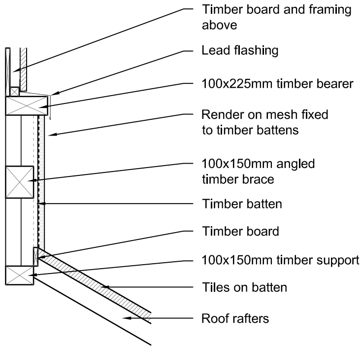
Existing Render Detail
