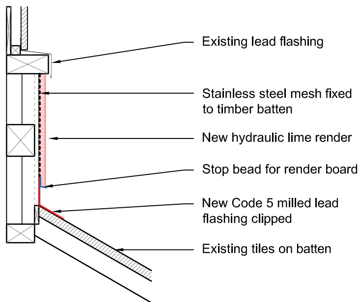
Proposed Render Detail
