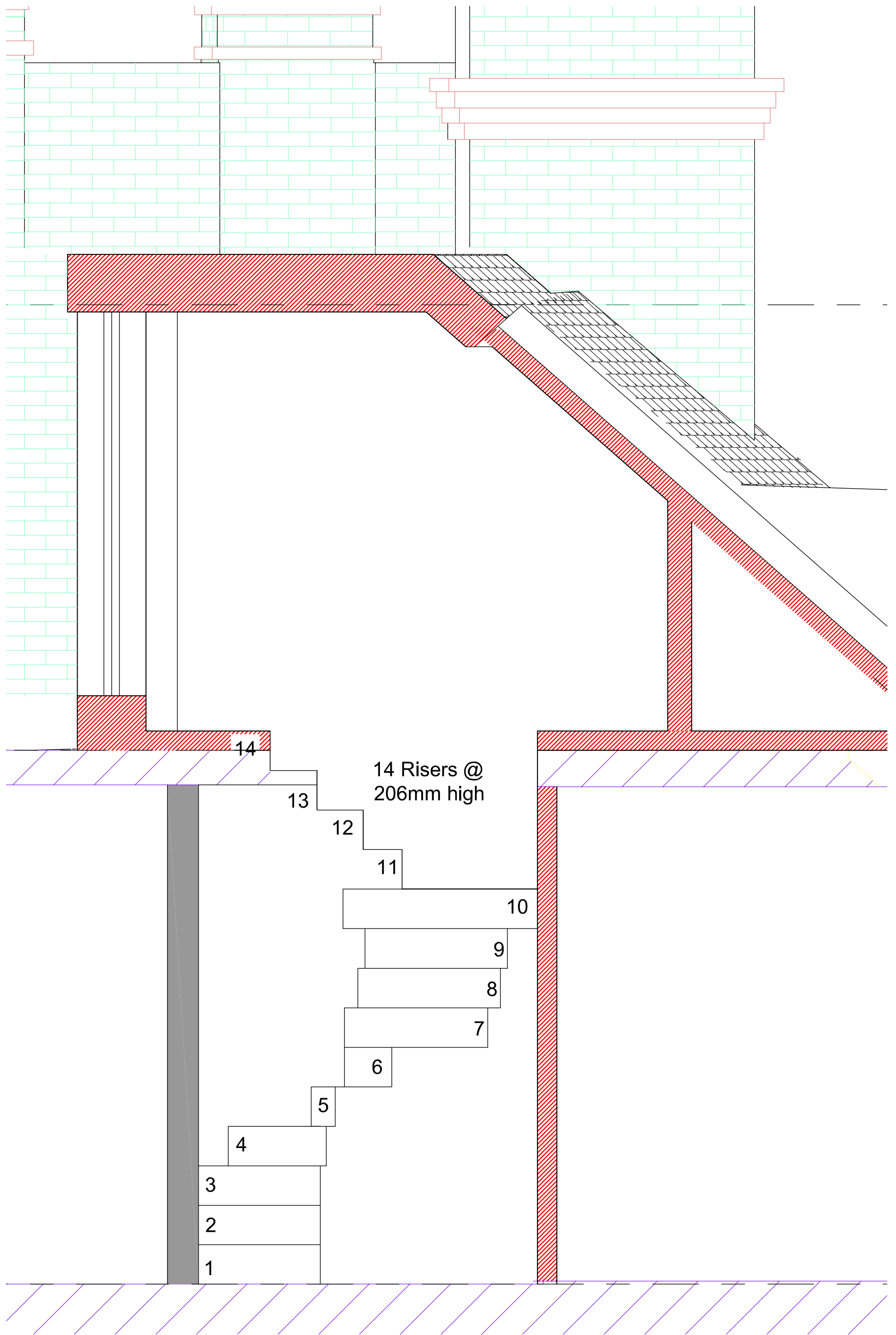
Proposed Staircase Section B-B
