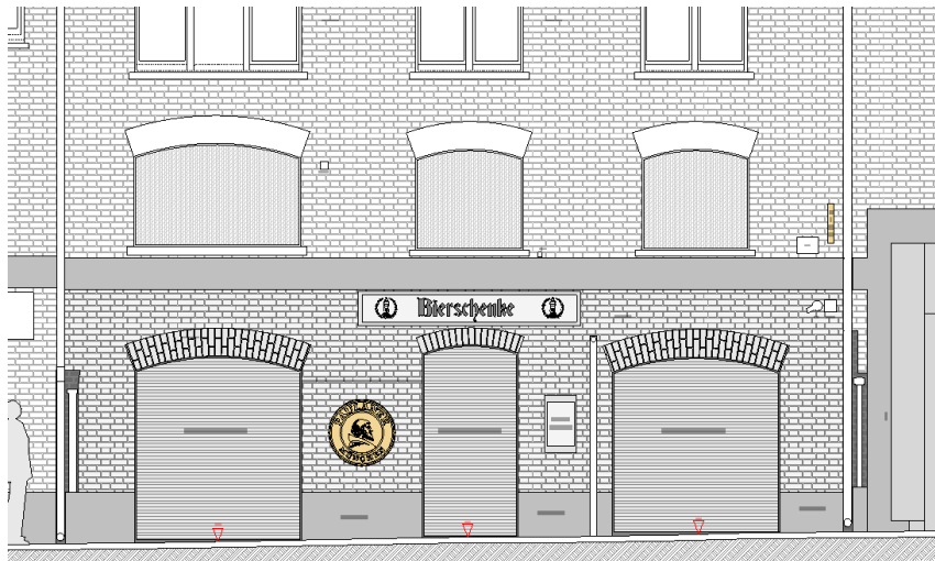
Earlham Street Elevation
