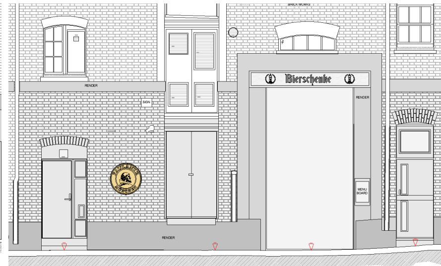
Shelton Street Elevation
