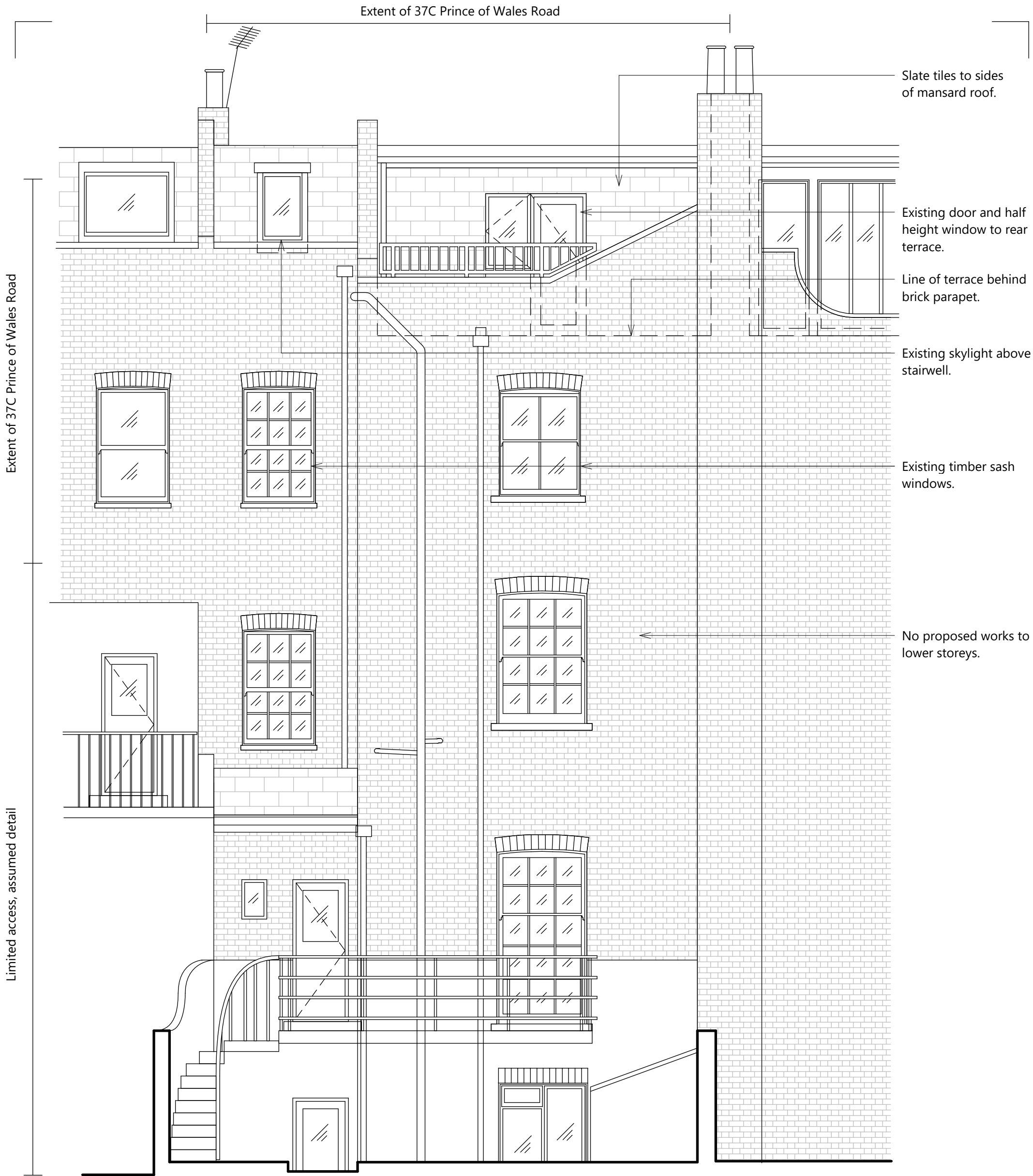
1 Existing South Elevation (Rear) 1 : 50
