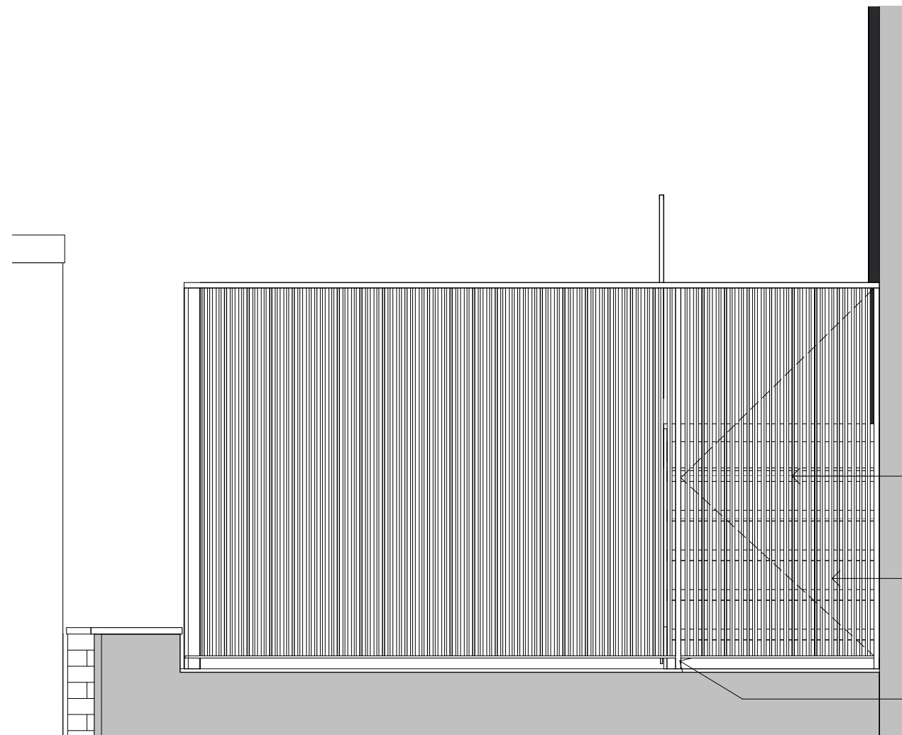
2 Elevation of Flat 23 privacy screen Scale: 1 : 25
