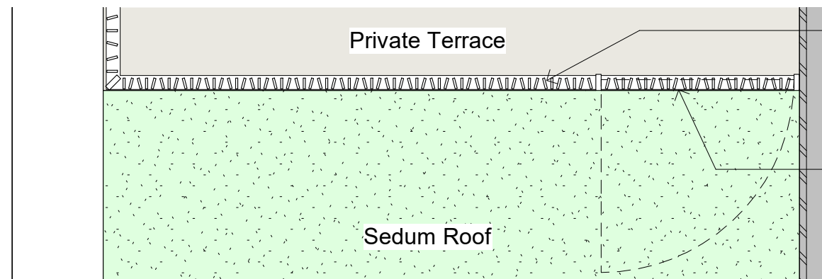
1 Plan of Flat 23 privacy screen Scale: 1 : 25
