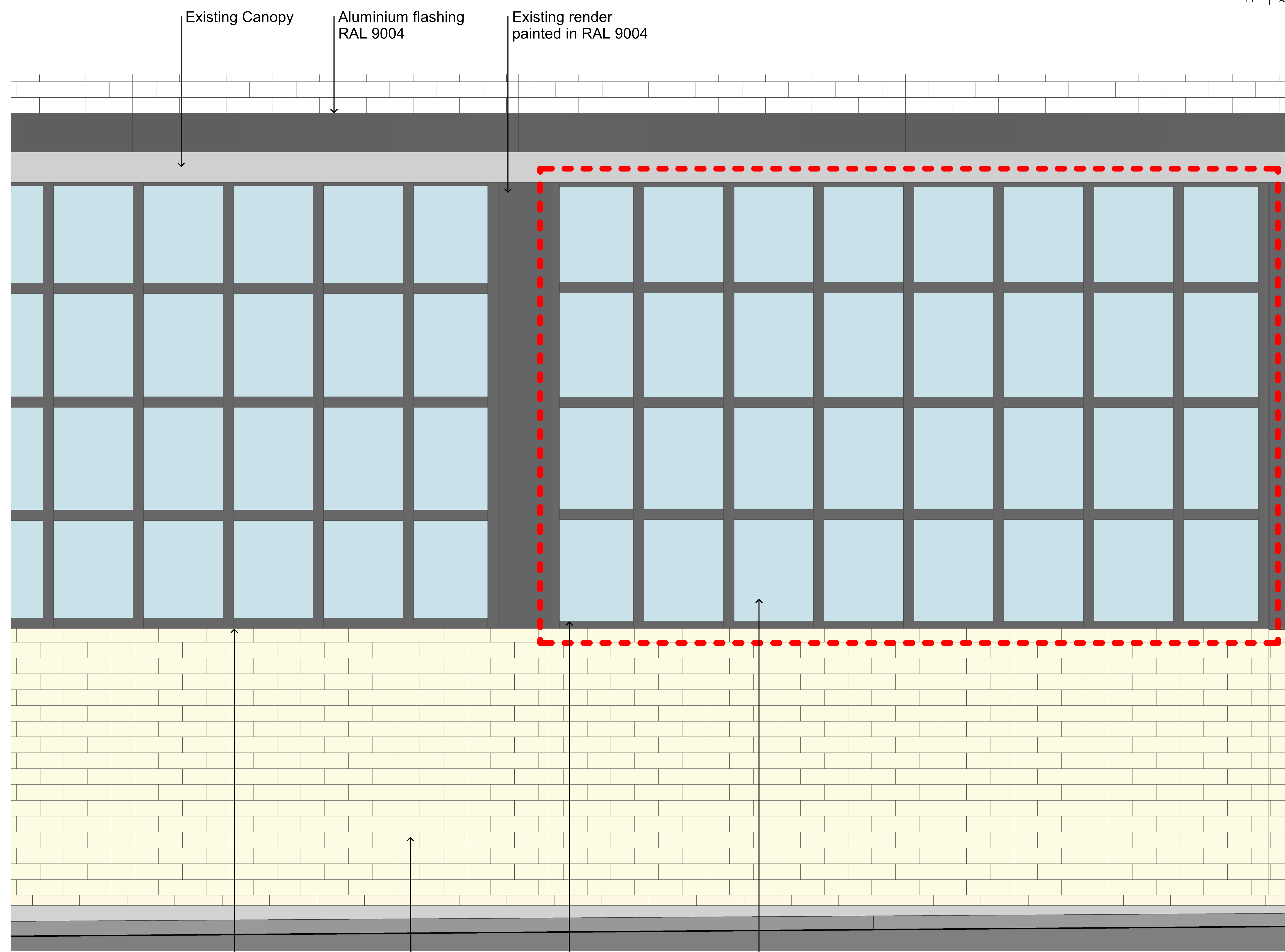
1 Field Street Windows Scale: 1 : 10
