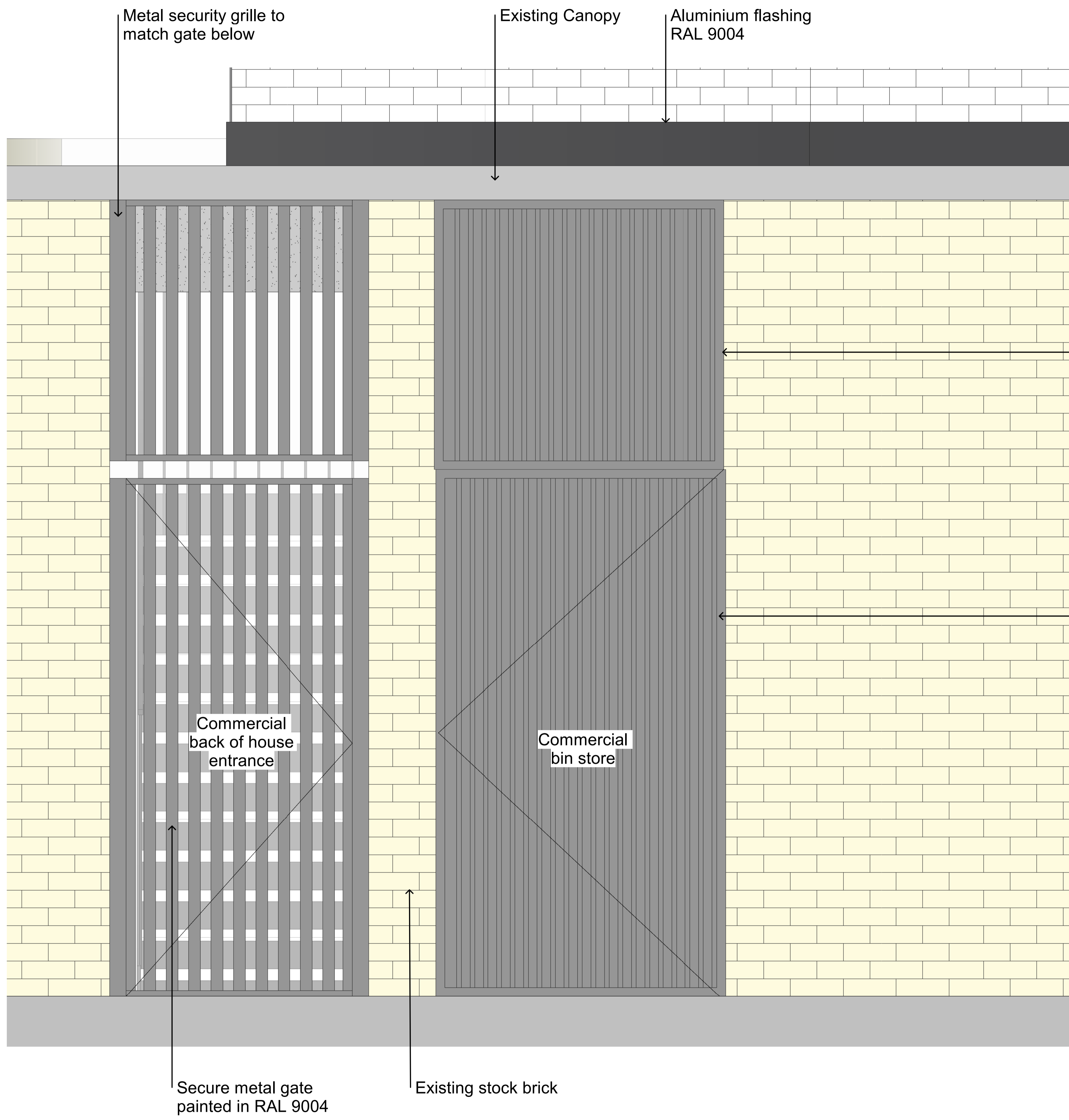
1 Field Street commercial back of house entrance Scale: 1 : 10
