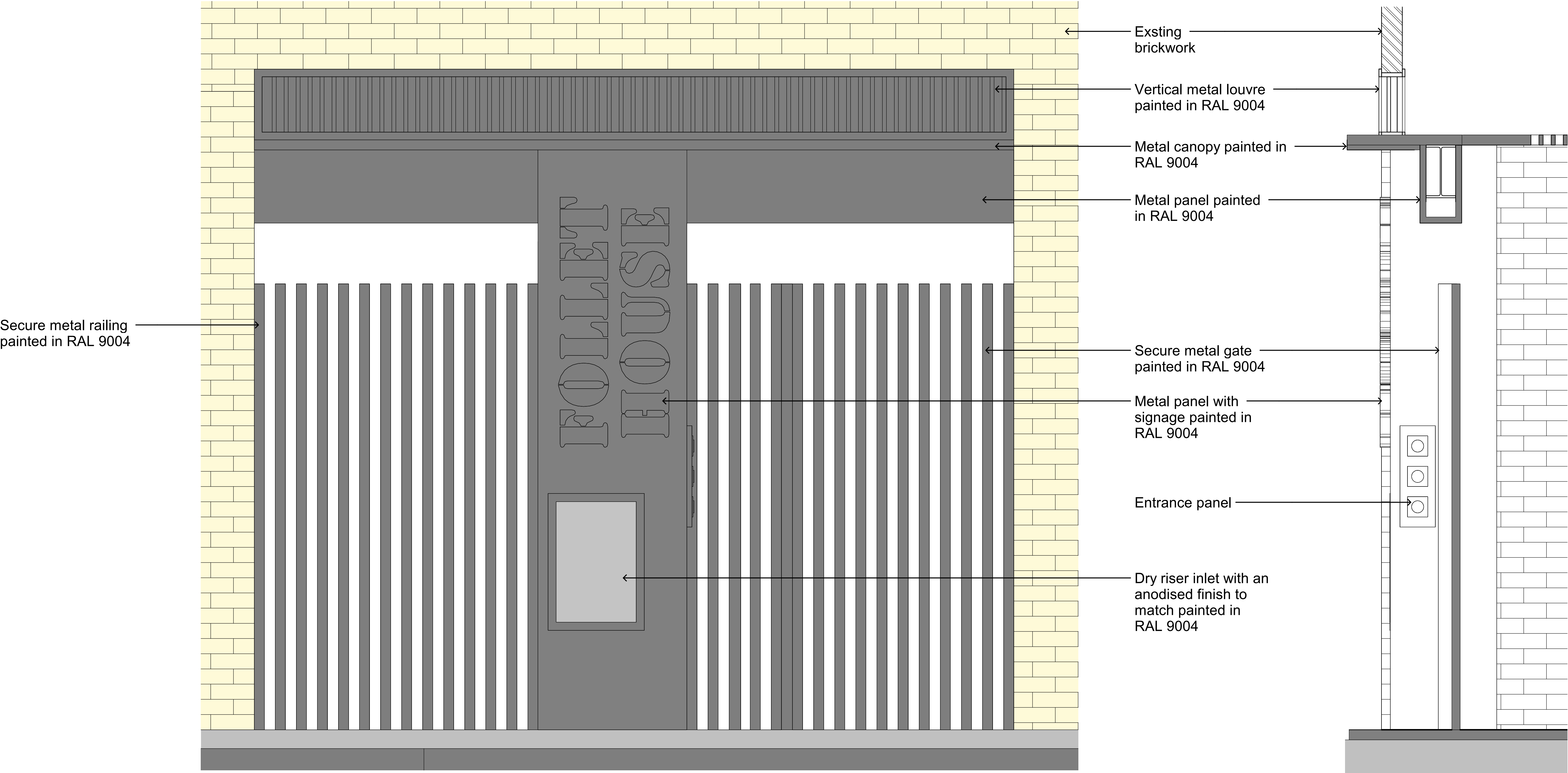
1 Leeke Street Residential Frontage Scale: 1 : 10
