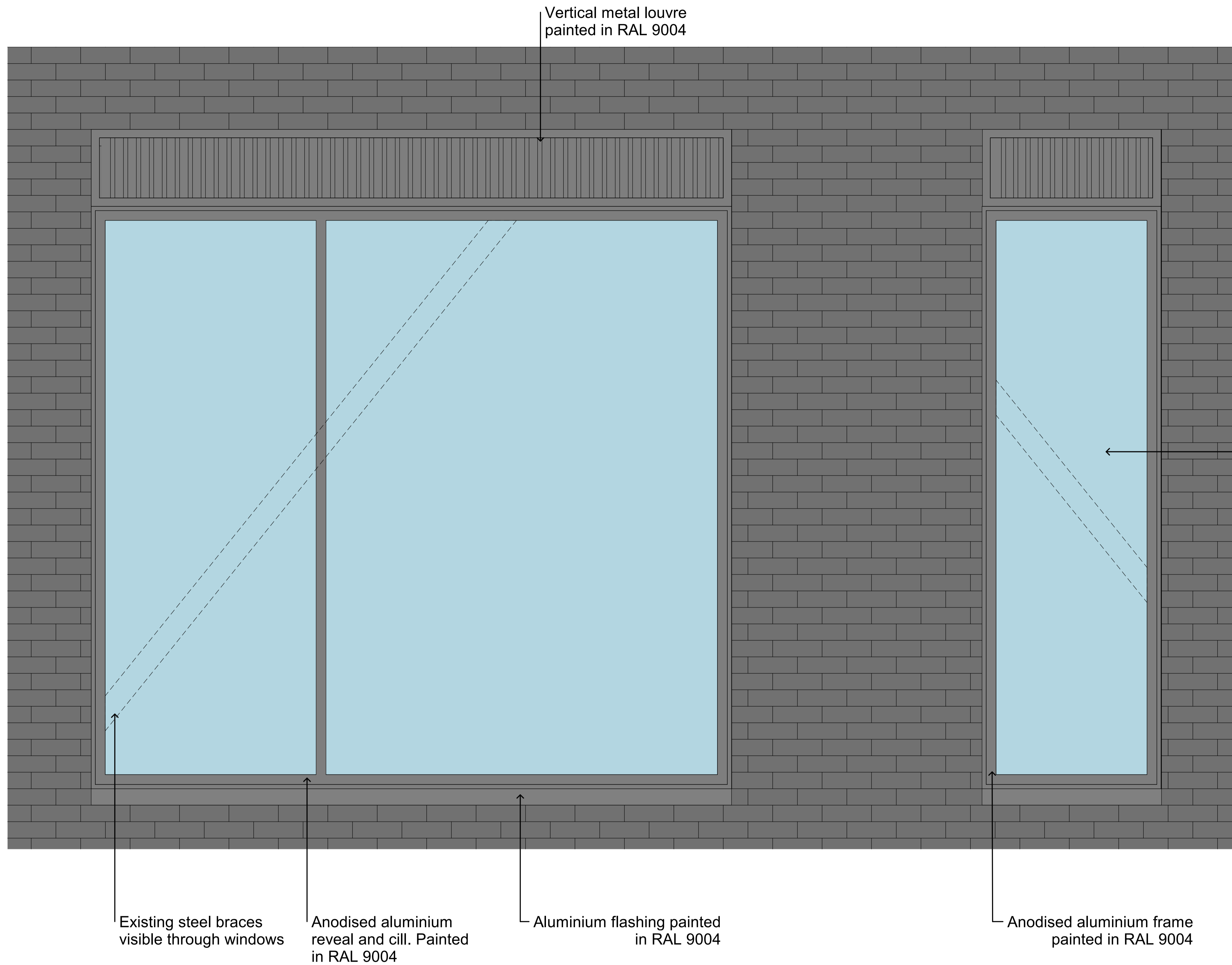
1 First Floor Leeke Street Windows Scale: 1 : 10
