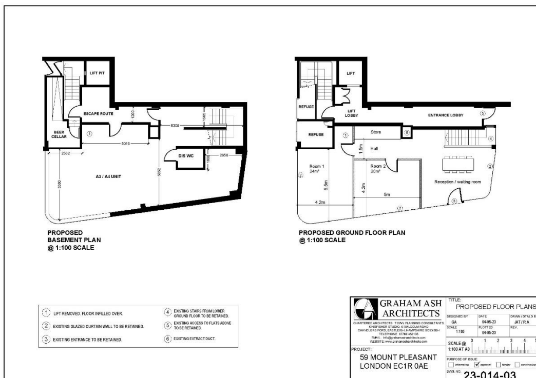
4.06 PROPOSED FLOOR PLANS SHOWING LAYOUT OF MEDICAL CENTRE
