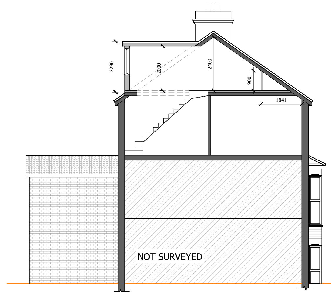
PROPOSED SECTION
