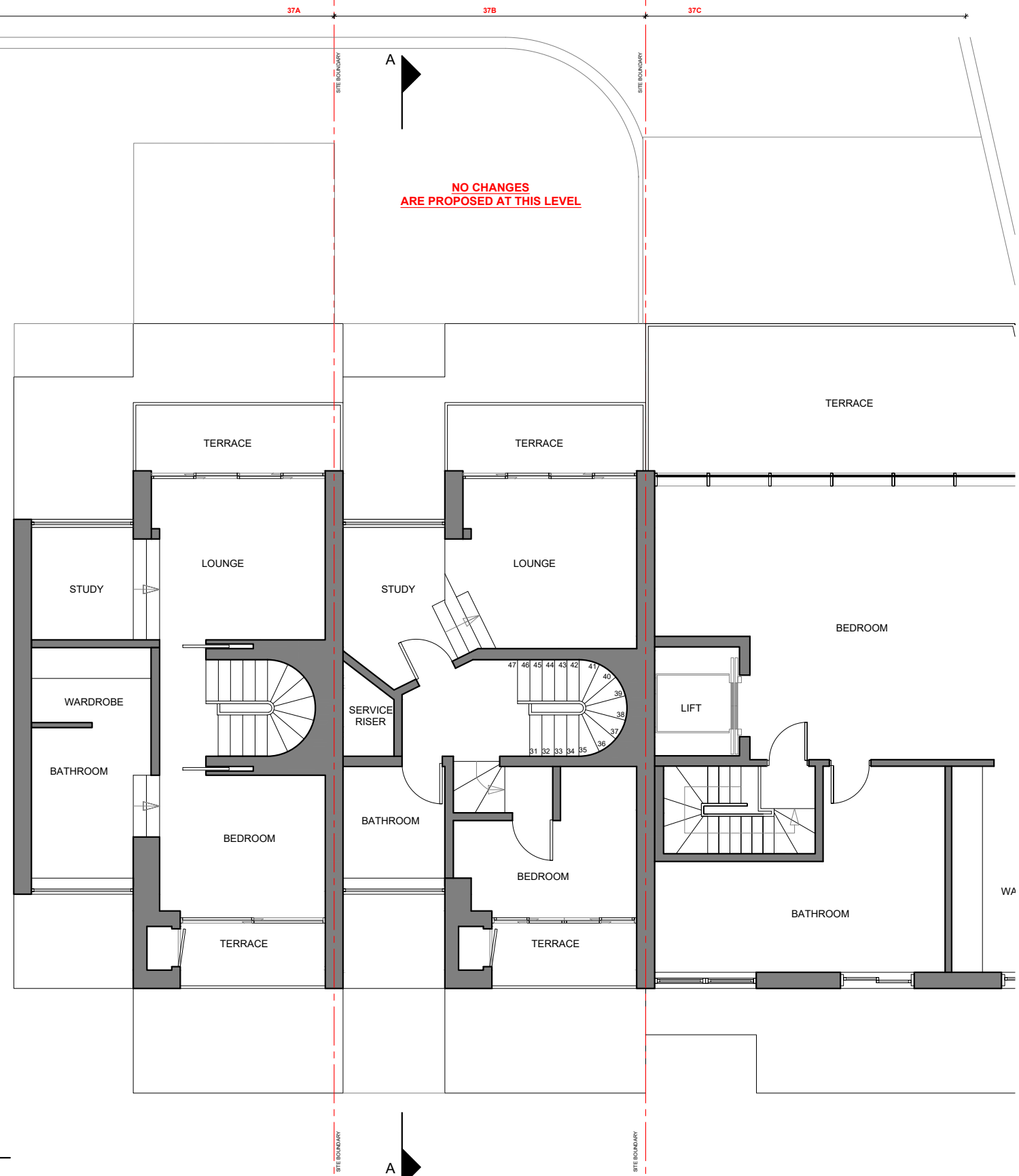
1 THIRD FLOOR PLAN - PROPOSED_ SCALE 1:100 @ A3
