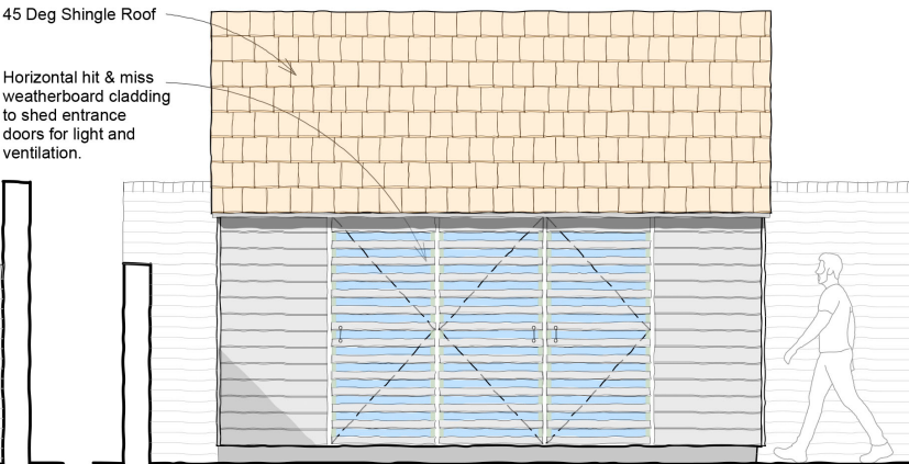
WEST ELEVATION- 1:50 (CLOSED SHED DOORS)
