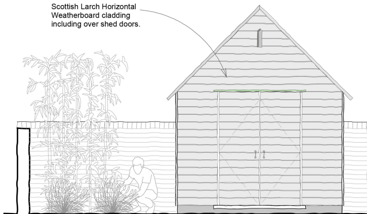
SOUTH ELEVATION- 1:50 (CLOSED SHED DOORS)
