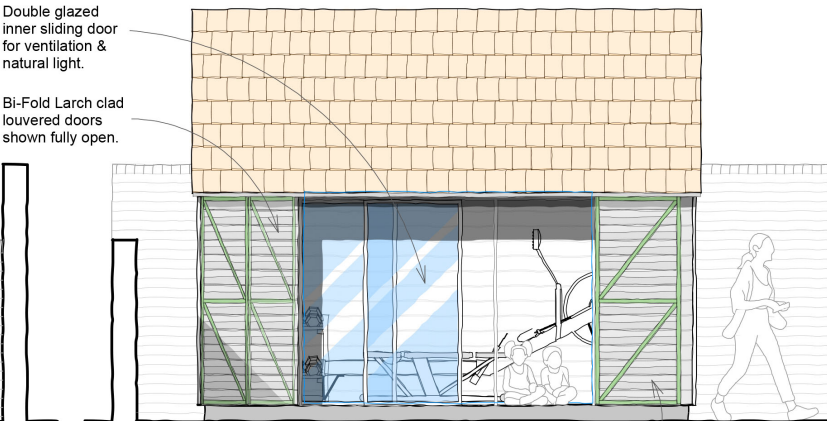
WEST ELEVATION- 1:50 (OPEN SHED DOORS)
