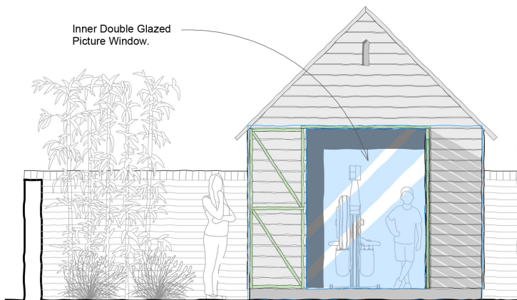
SOUTH ELEVATION- 1:50 (OPEN SHED DOORS)
