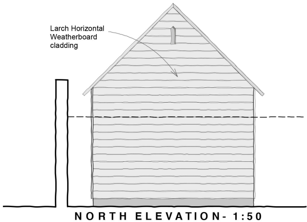
NORTH ELEVATION- 1:50
