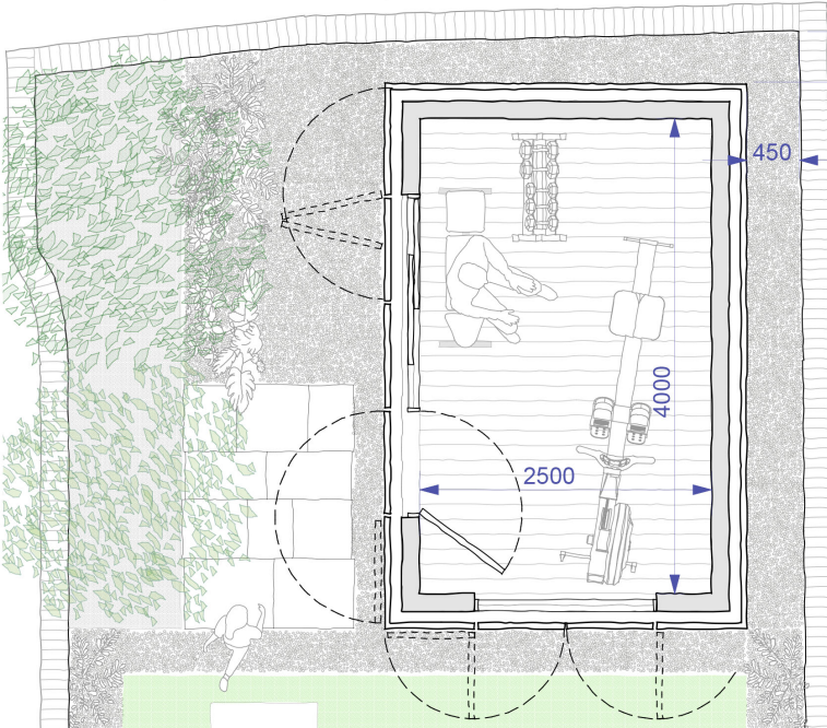
GARDEN SHED PLAN - 1:50
