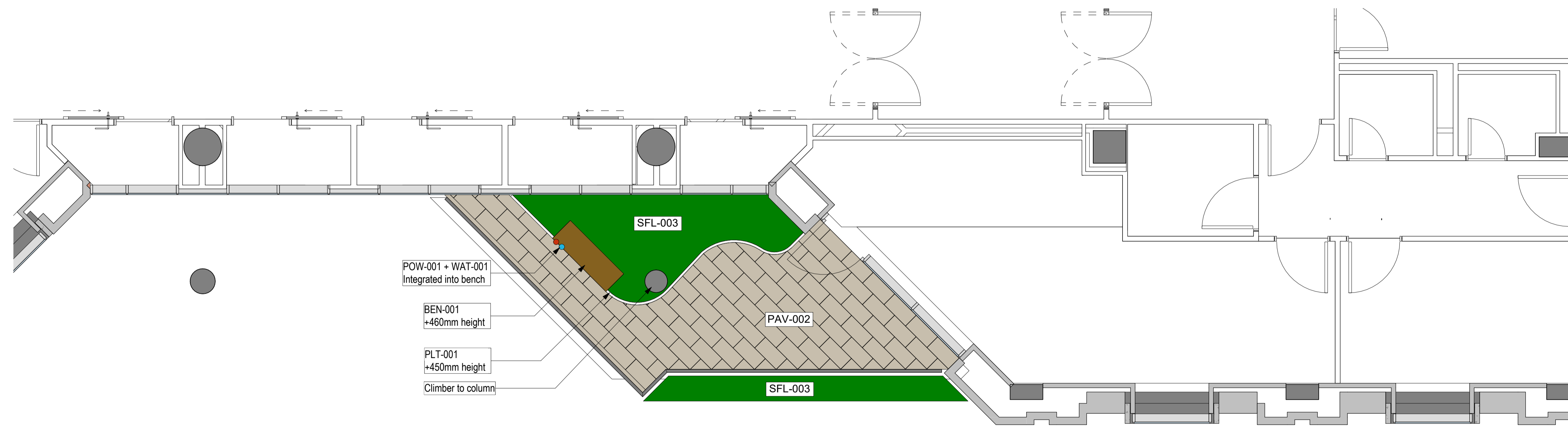
2 Level 3 Staff Balcony 1 : 50
