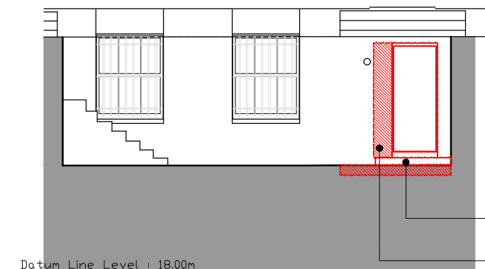
5 Demolition Elevation 02 GHV 1:100 @ A3
