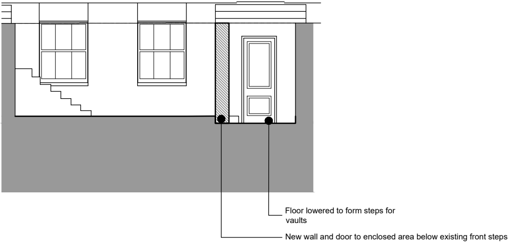
2 Proposed Elevation 02 GHV 1:100 @ A3
