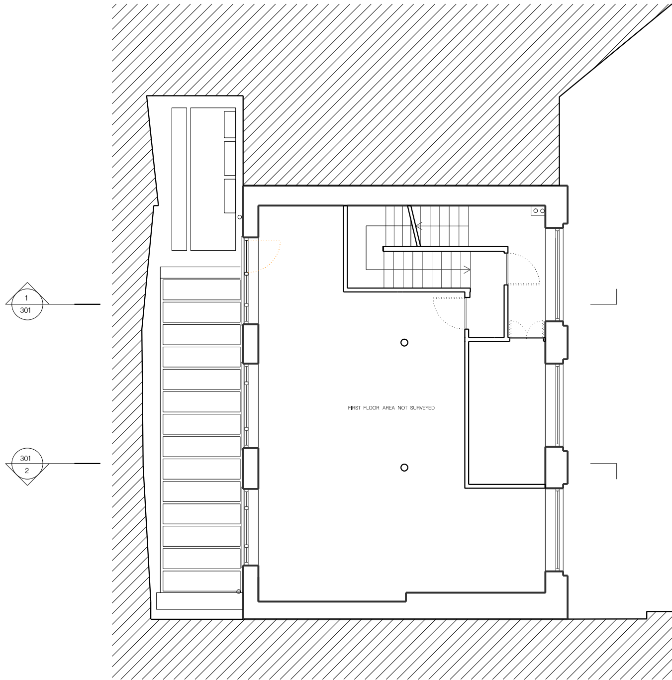
① EXISTING FIRST FLOOR PLAN
