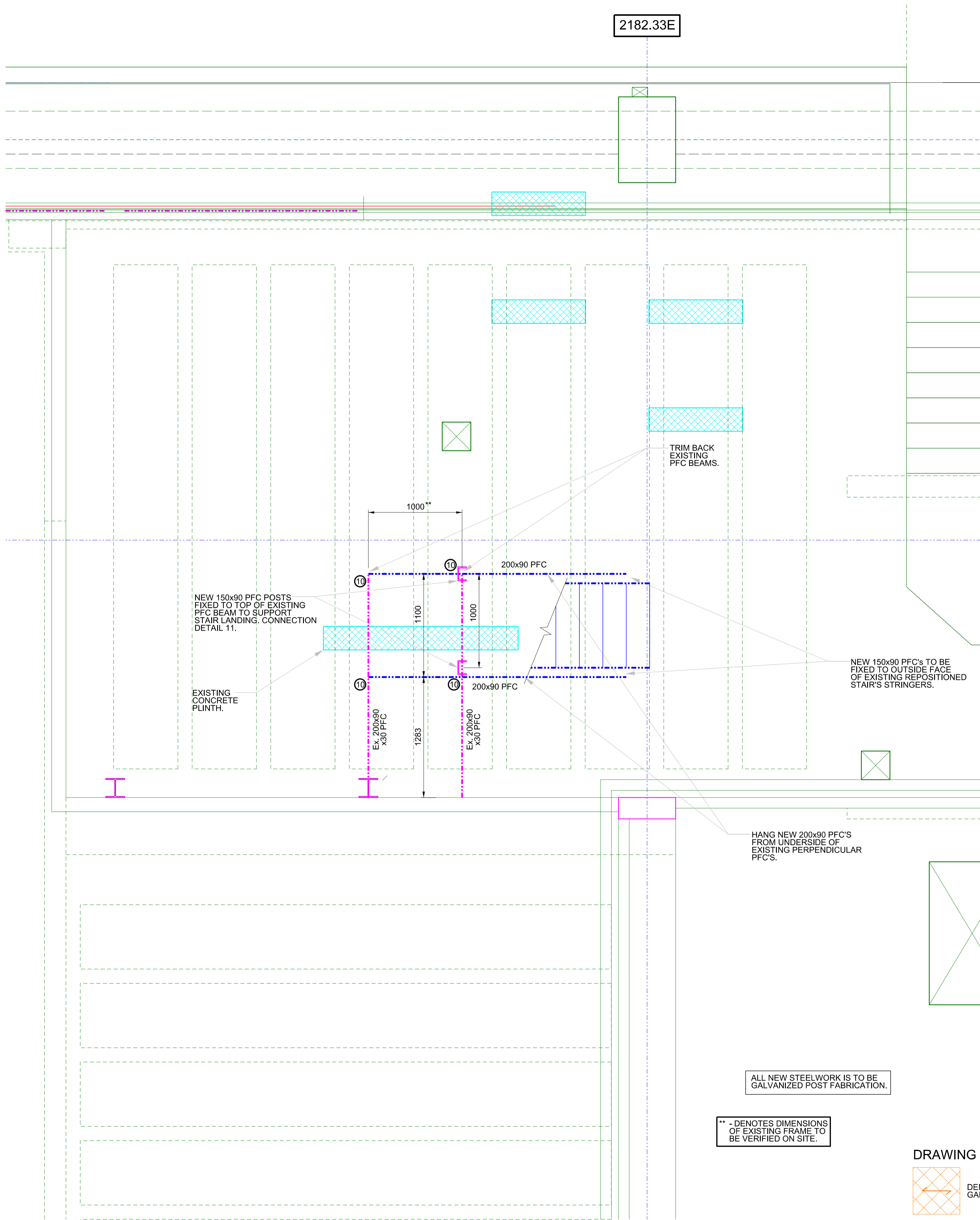
LOW LEVEL PLAN AT ROOF LEVEL
