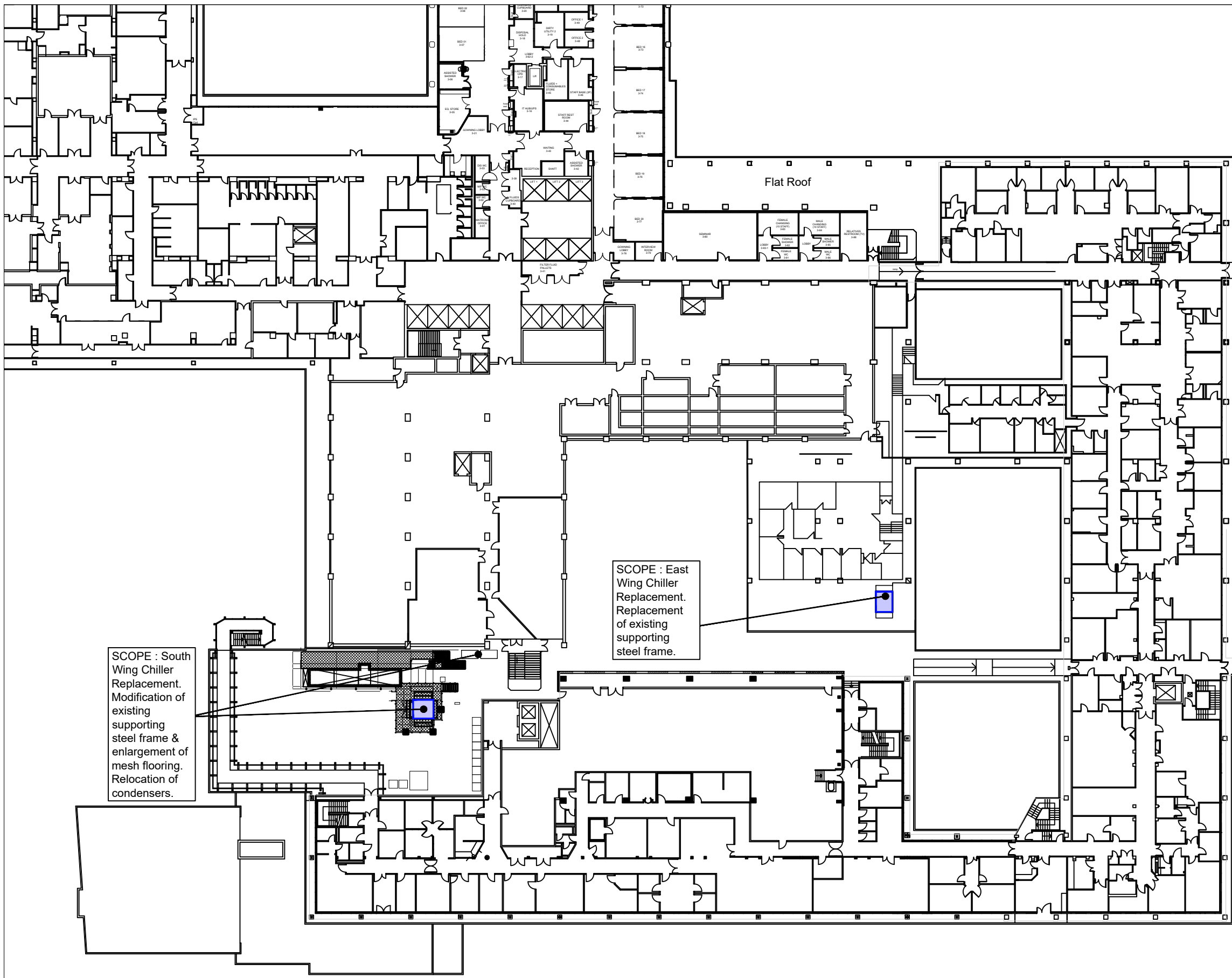
01 Proposed Level 3 Plan (01)003 1:500 @ A3
