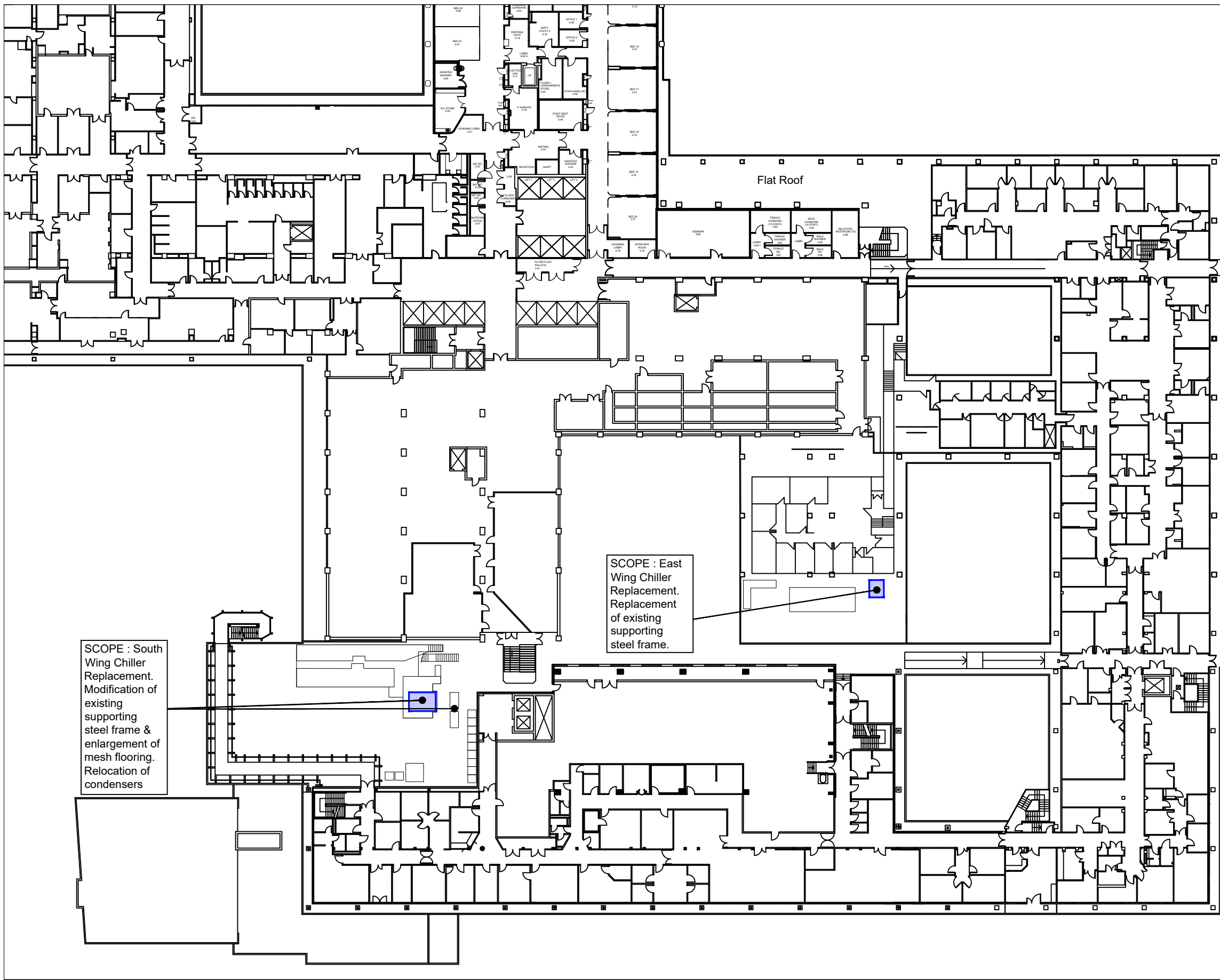
01 Existing Level 3 Plan-South & East Wing Chiller (01)001 1:500 @ A3
