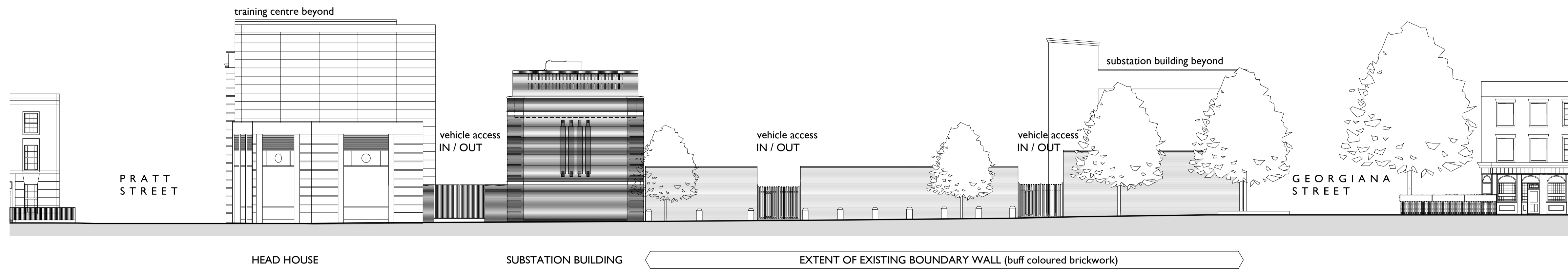
EXISTING ROYAL COLLEGE STREET ELEVATION - A _ Scale 1:200 @ A1
