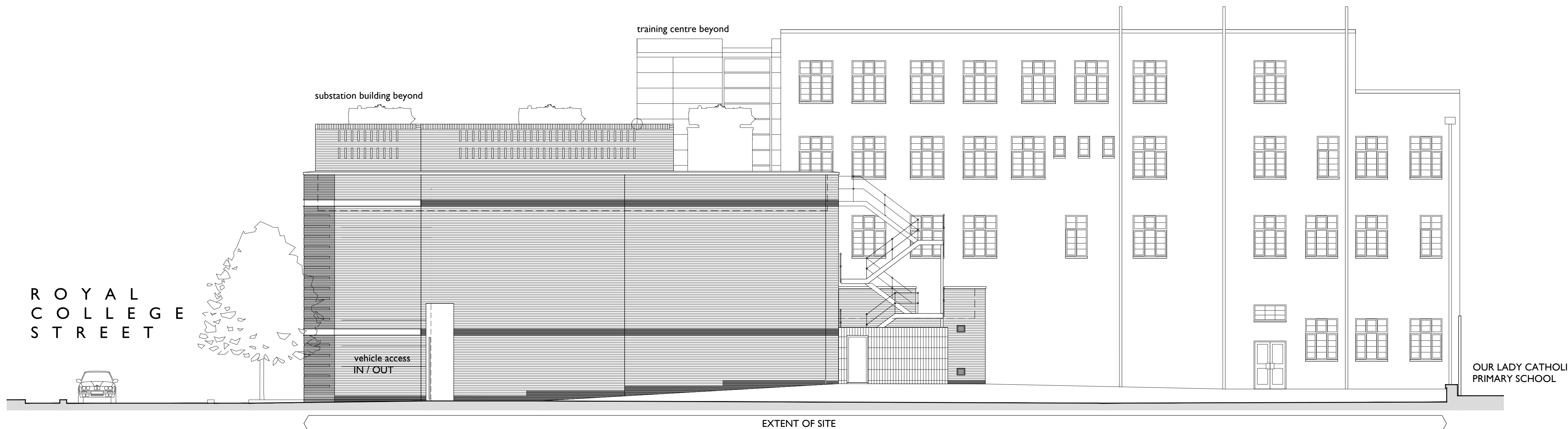
EXISTING SECTION B - B _ Scale 1:100 @ A1
