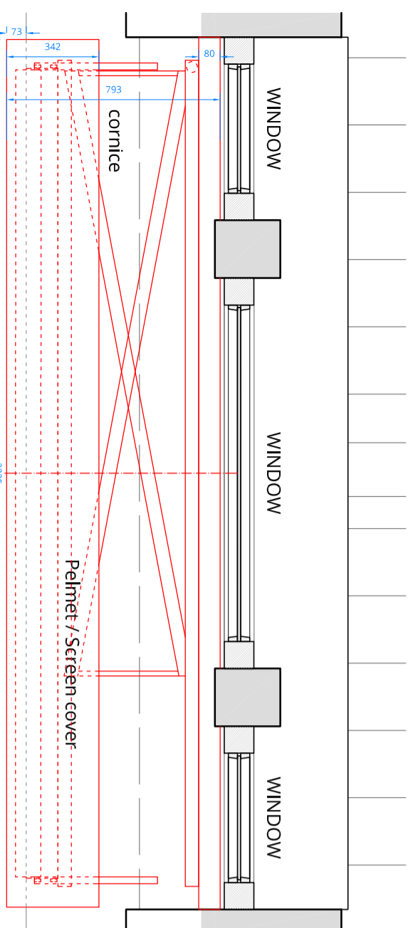
Proposed Screen System - Plan - Open
