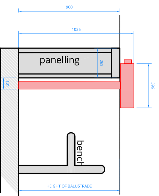
Projector Section
