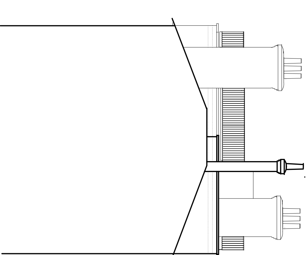
NORTH END ELEVATION AS EXISTING
