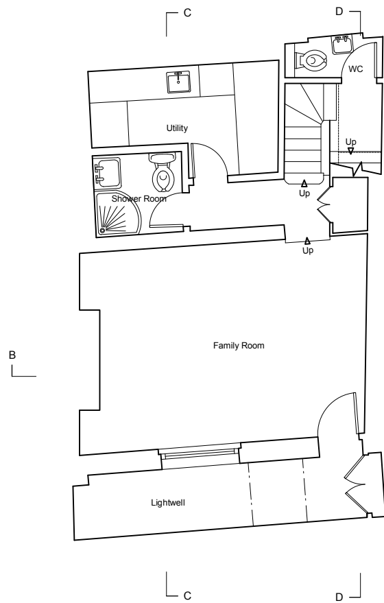
EXISTING LOWER GROUND FLOOR PLAN
