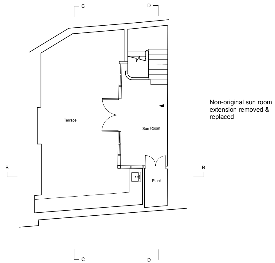
EXISTING FOURTH FLOOR PLAN
