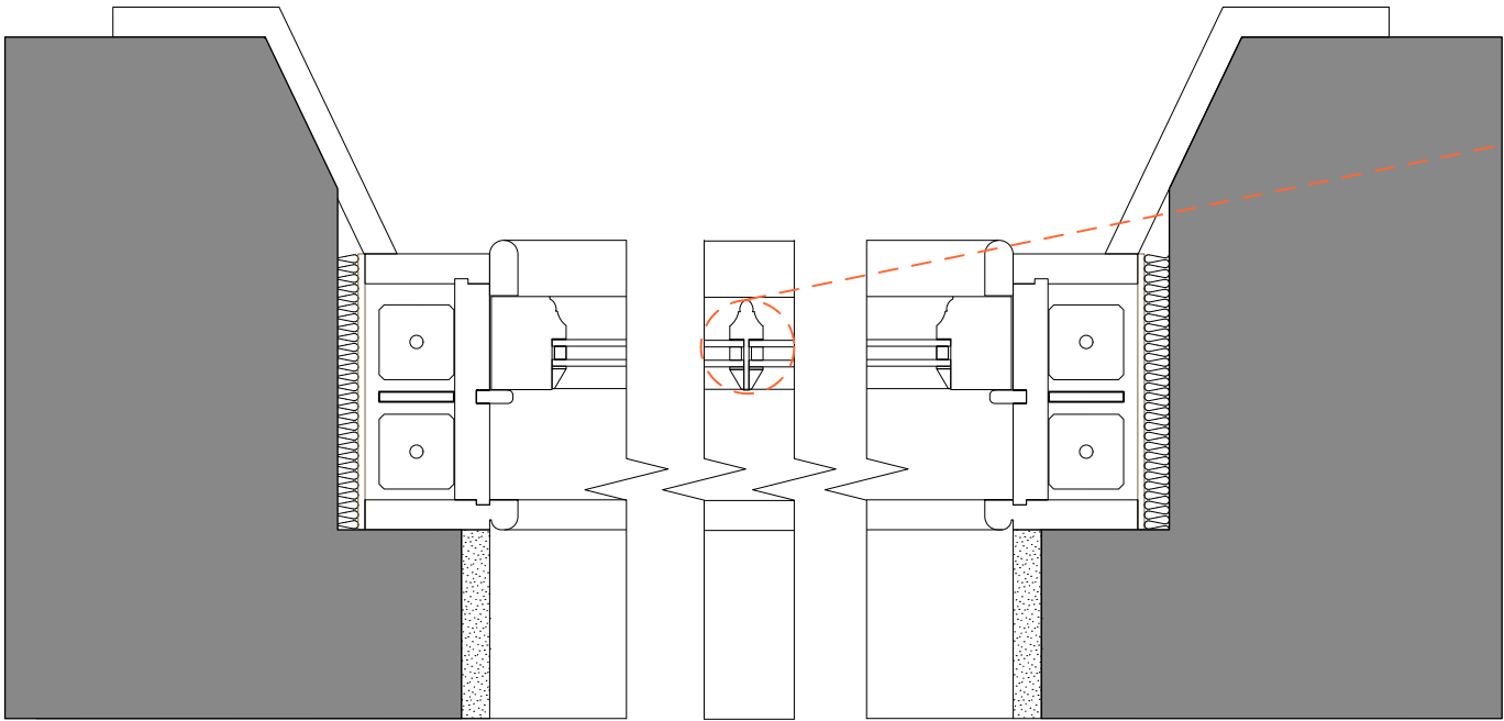
P Proposed Standard Sash Window Plan 1:5
