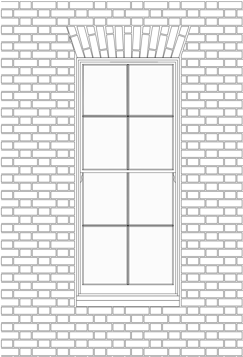
E Proposed Standard Sash Window 1:20
