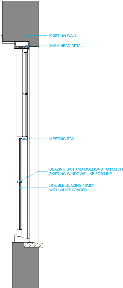
S Proposed Standard Sash Window Section 1:20
