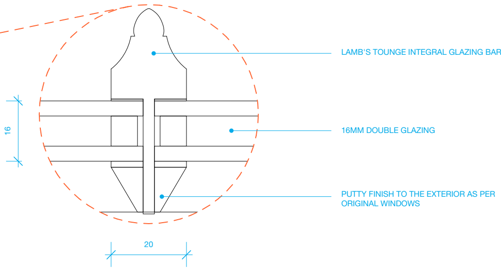
D Proposed Sash Window Glazing Bar Actual Size
