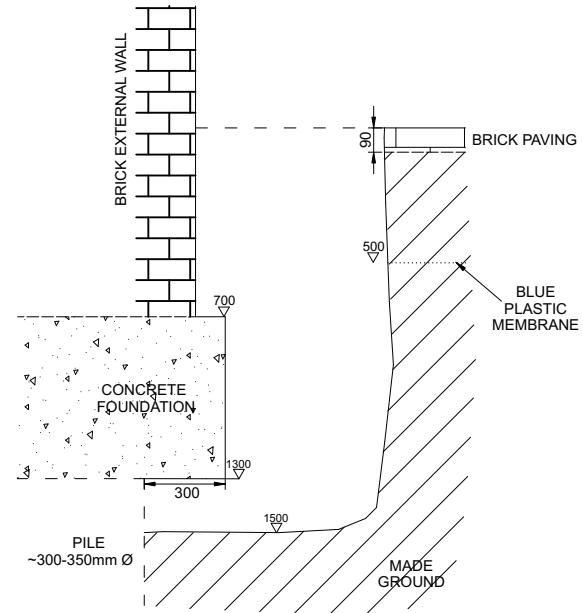
TP03 SECTION A-A'
