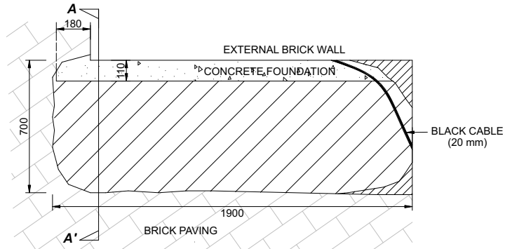
TP03 PLAN VIEW
