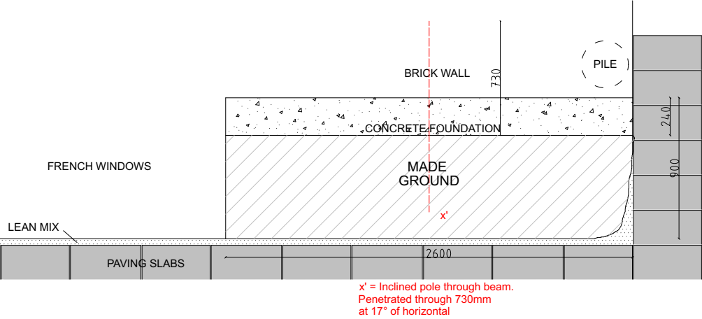
TP01 NORTH PLAN VIEW
